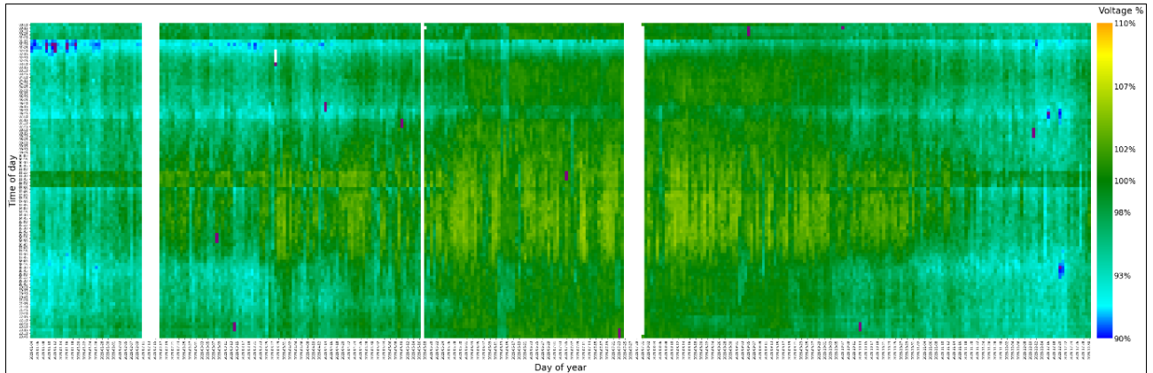
Fig. 2 – Calendar heatmap showing the voltage evolution for an end-customer affected by low voltage falls
