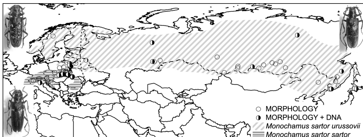
Fig. 1. Distribution of Monochamus sartor sartor and M. s. urussovii in Eurasia with localization of sampling sites for morphological and molecular studies. Broken line – approximate border between eastern and western populations of M. s. urussovii .
