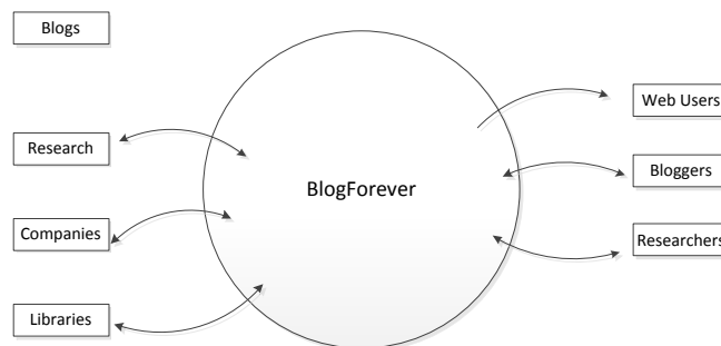
Figure 19 - BlogForever Data Flow: Context Diagram
