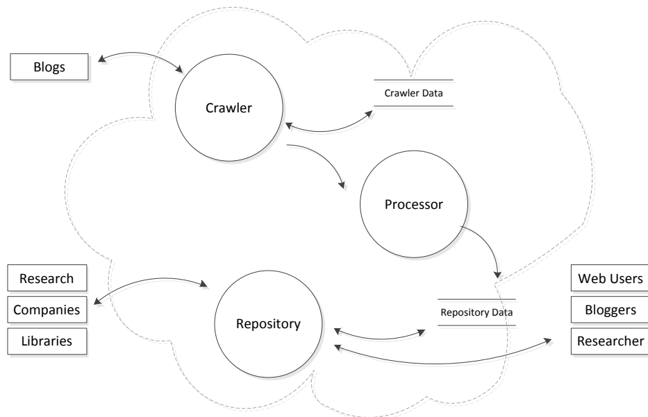
Figure 20 - Data flow diagram at level 1
