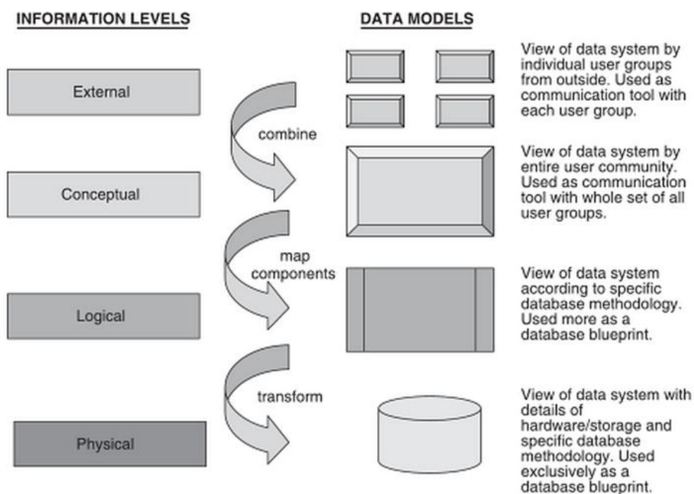
Figure 1 - Data models at different information levels (from Ponniah et. al [4], p. 14).
