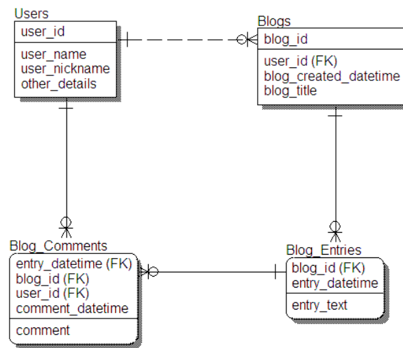
Figure 9 - Generic and simple data model for blogs (from Williams [21]).
