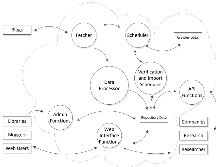
Figure 21 - Data flow diagram at level 2.
