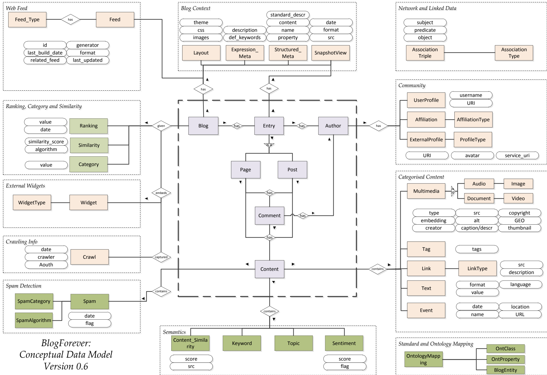
Figure 17 – Conceptual data model for blogs.
