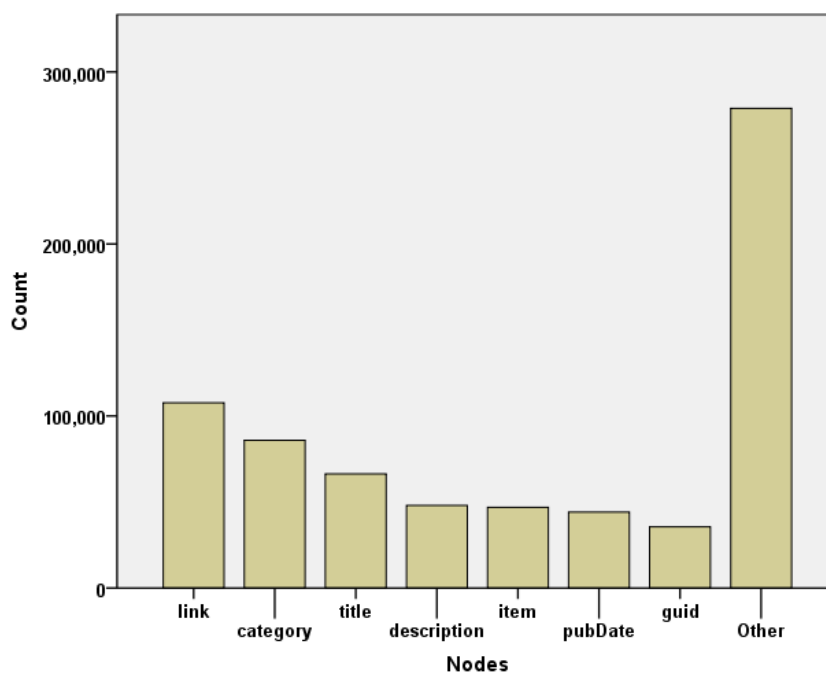
Figure 14 - Most frequently used nodes in web feeds (3% of cases collapsed).
