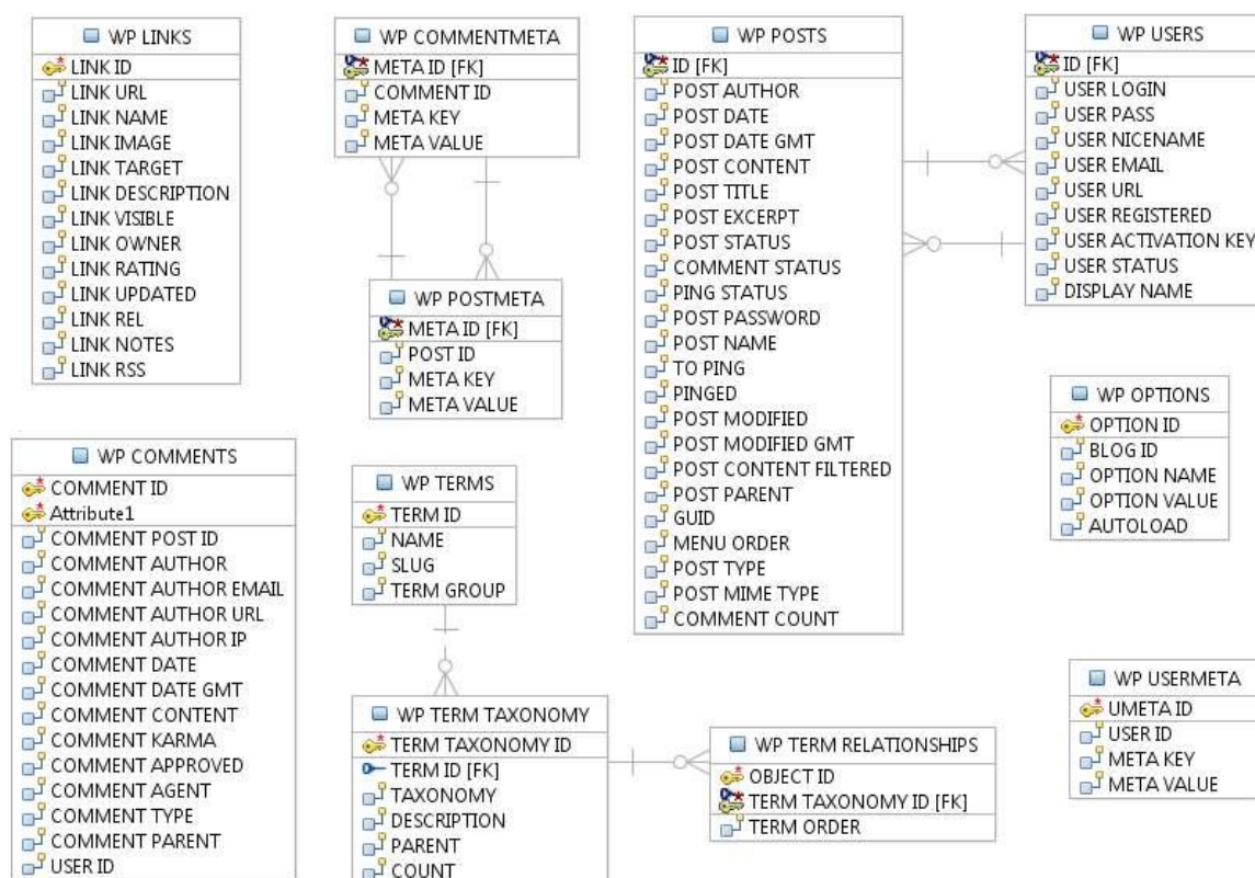
Figure 10 - Entity relationship model reflecting the database structure of a default installation of WordPress 3.2.1 software.
