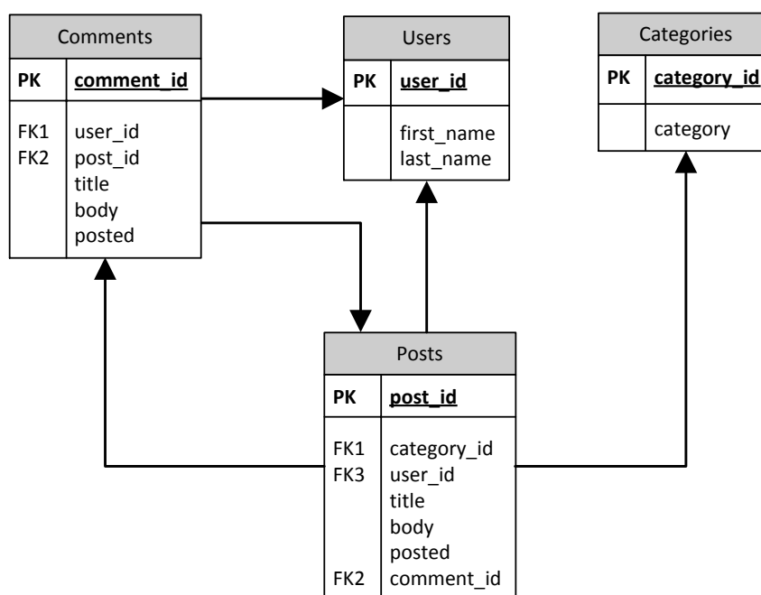
Figure 8: Entity relationship model for a simple blog.
