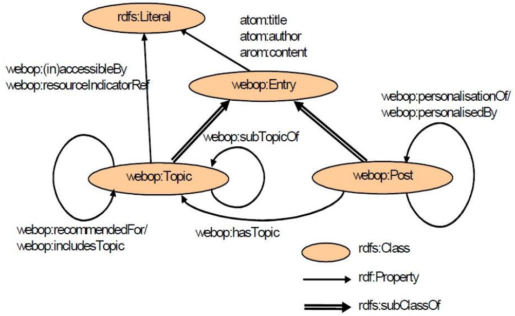
Figure 7 - Blog model (from Ta et. al [18]).
