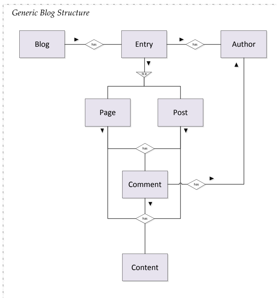
Figure 16 - Generic blog data model
