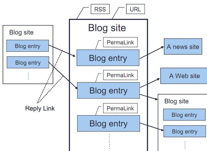
Figure 3 - Conceptual model of a blog at a website level (from Nakajima et. al [17]).
