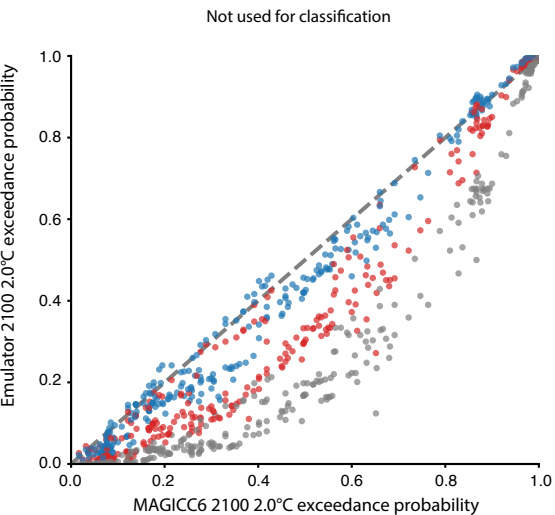
c 2100 2.0°C exceedance probability
