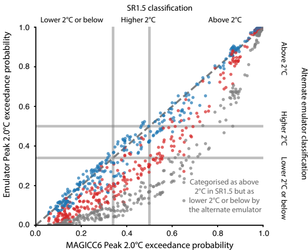
d Peak 2.0°C exceedance probability
