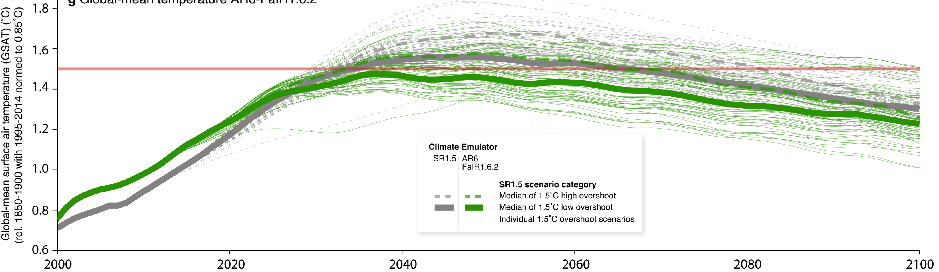
g Global-mean temperature AR6-FalR1.6.2
