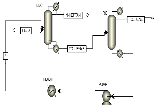
Figure 3. Extractive distillation process flowsheet for separating n-heptane from toluene using either sulfolane or [4EMPy] [NTF 2 ] as an entrainer
