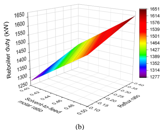
Figure 6. Effect of the solvent-to-feed molar ratio and the reflux ratio on the reboiler duty using sulfolane (a) and [4EMPy] [NTF 2 ] (b)
