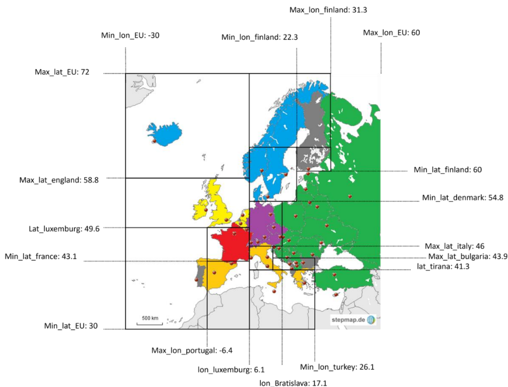
Figure 32: Areas of Eeuropean cities for attribution of monthly factors.
