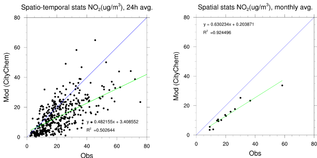
Figure 21: Regression plots of modelled \text{NO}_2 concentration versus monitored \text{NO}_2 concentration when including 14 monitoring stations in Hamburg using (a) 24-hour averages and (b) monthly averages. Blue line denotes the 1:1 line and the green line is the regression line. Regression parameters are included in the plots.
