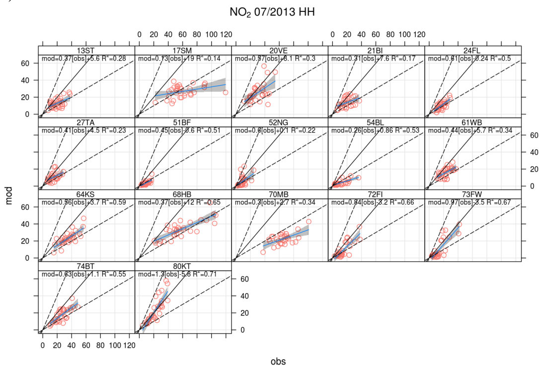
Figure 25: OpenAir scatterplot of (a) monthly averaged data and (b) daily averaged data, grouped by station. The analysis with OpenAir includes all available 17 monitoring stations in Hamburg.
