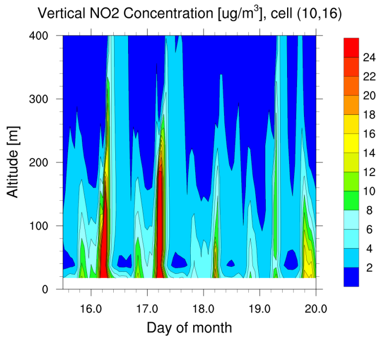
Figure 16: Hourly time slices of the vertical profile of NO 2 mixing ratio (in \mu\text{g}/\text{m}^3 ) for main grid cell (10,16) for 4.5 days in July 2013 (starting at noon of 15 th July) as contour plot created by routine vertical_profile.ncl .
