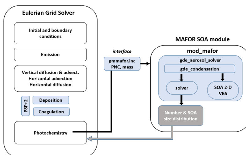
Figure 3: Block structure of the Eulerian grid solver with P8P+2 and the MAFOR-SOA module in EPISODE-CityChem. The new modules are in blue shaded blocks.
