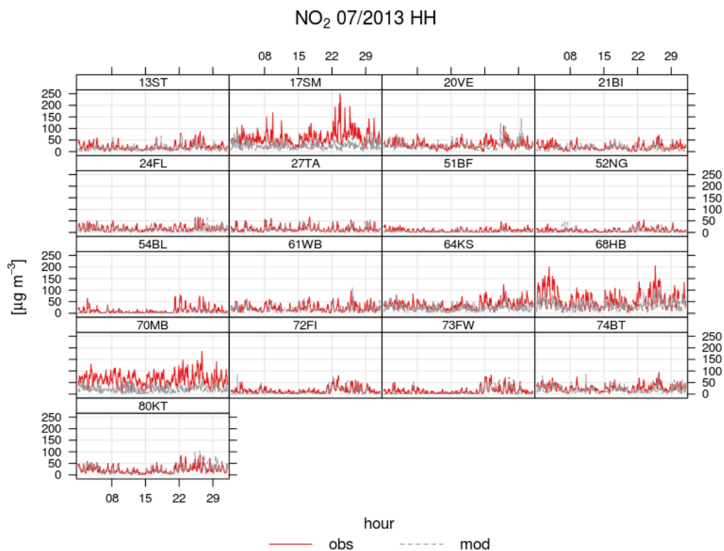
Figure 22: OpenAir time series plots generated by timePlot for observed and modelled data grouped by station.
