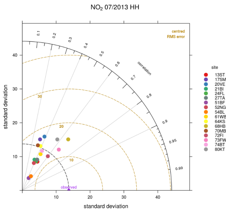
Figure 24: OpenAir generated Taylor diagram of observed and modelled data, grouped by stations.
