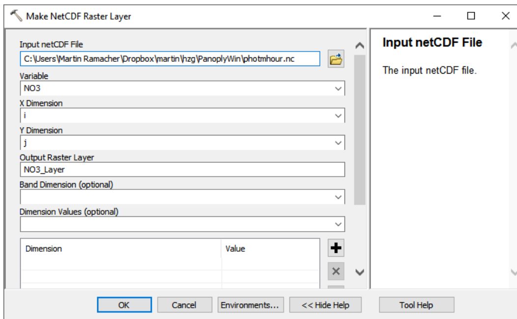
Figure 28: Make netCDF file tool with exemplary inputs.
