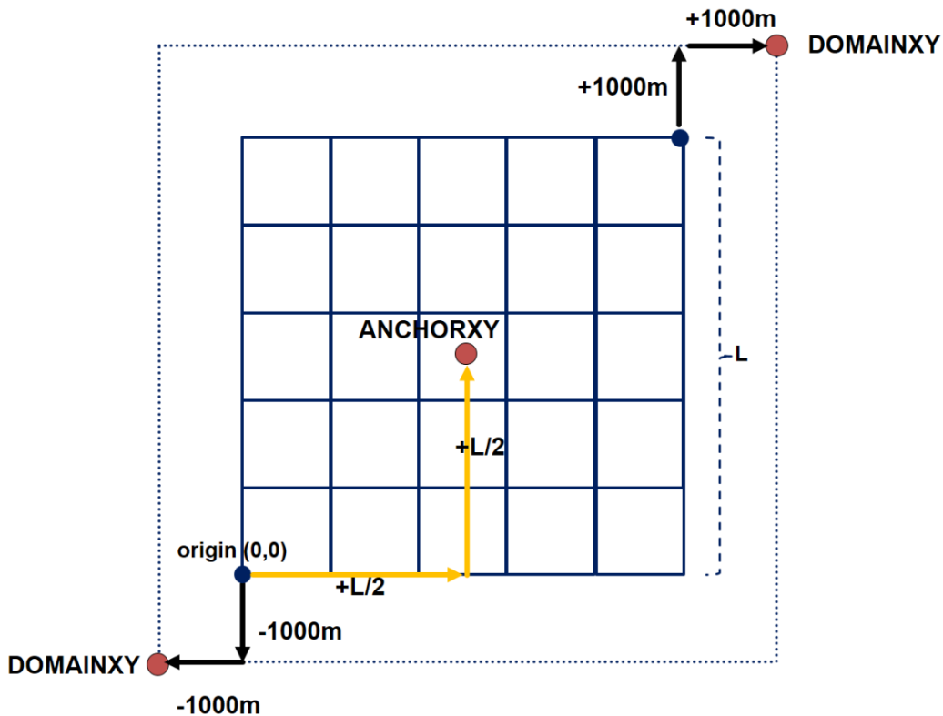
Figure 11: Illustration of the grid definition in AERMAP.
