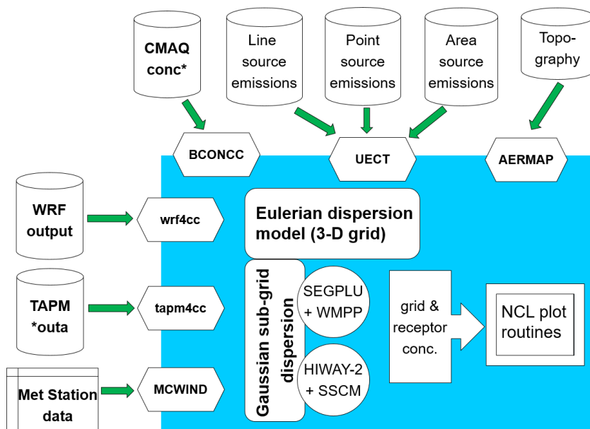
Figure 4: Overview of EPISODE-CityChem model components: utilities and interfaces.
