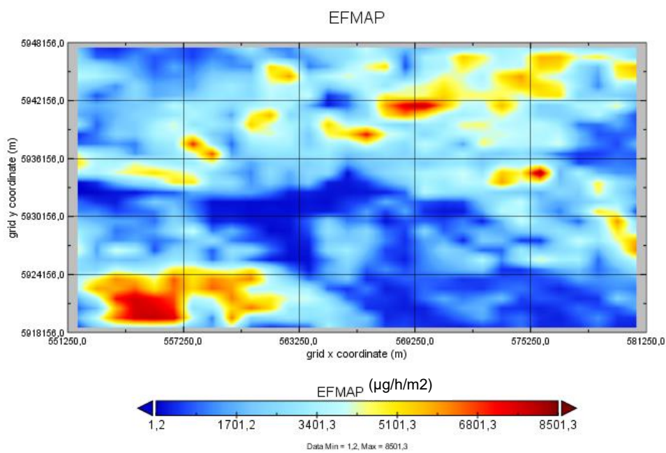
Figure 34: Map of isoprene emission factors for the region of Hamburg: a) isoprene standard emission potential (unit: \mu\text{g}/\text{g}/\text{hr} ) map created based on Copernicus Tree Cover Density and Corine Land Cover; resolution of 100 m; b) interpolated field of emission factor \times foliar density (unit: \mu\text{g}/\text{hr}/\text{m}^2 ) calculated in UECT; resolution of 1000 m in zoom region of a).
