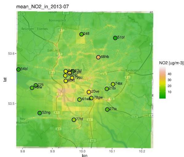
Figure 26: Spatial map of NO 2 monthly concentration average (in \mu\text{g m}^{-3} ) for Hamburg city plotted with the routine create_ggmap.R . Open black circles denote stations.
