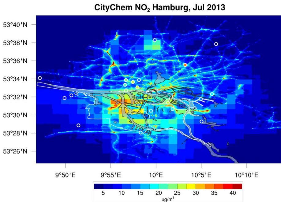
Figure 14: Spatial map of NO 2 monthly concentration average (in \mu\text{g m}^{-3} ) for Hamburg city plotted with the routine create_map.ncl . White outline illustrates harbour areas and black outline illustrates water bodies. Open white circles denote stations.
