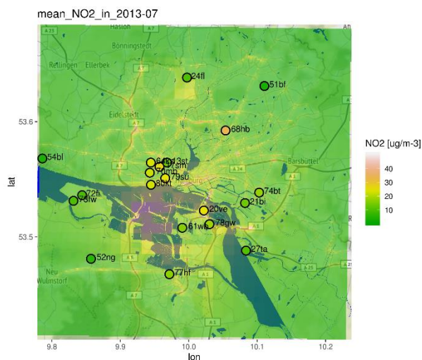
Figure 27: Spatial map of NO 2 monthly concentration average (in \mu\text{g m}^{-3} ) for Hamburg city plotted with the routine create_ggmap.R . Open black circles denote stations. Blue areas in the background display port areas and water bodies, which are derived from Urban Atlas.
