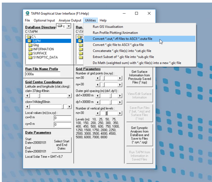
Figure 6: TAPM Graphical User Interface, selection of outa-file creation in the Utilities menu.
