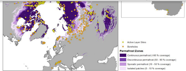
Figure 1: Location of the GTN-P PT (orange dots) and ALT (yellow dots) monitoring sites and permafrost distribution. Permafrost Zones are based on Obu et al. 2019
