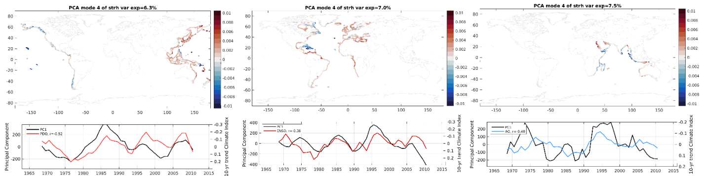
Figure S8. Steric PC4 spatial pattern (top) and rolling decadal trend (bottom).
