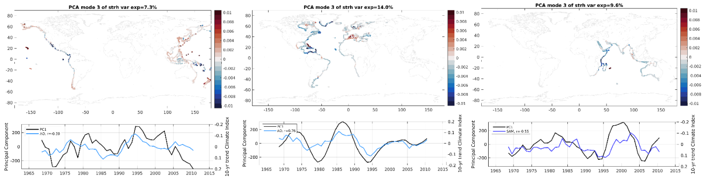
Figure S7. Steric PC3 spatial pattern (top) and rolling decadal trend (bottom).
