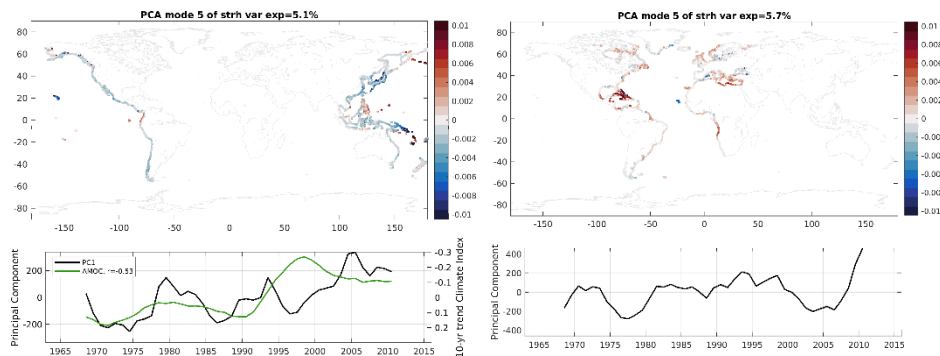
Figure S9. Steric PC5 spatial pattern (top) and rolling decadal trend (bottom). This pattern is ignored in the Atlantic and Indian basins in the reconstruction.
