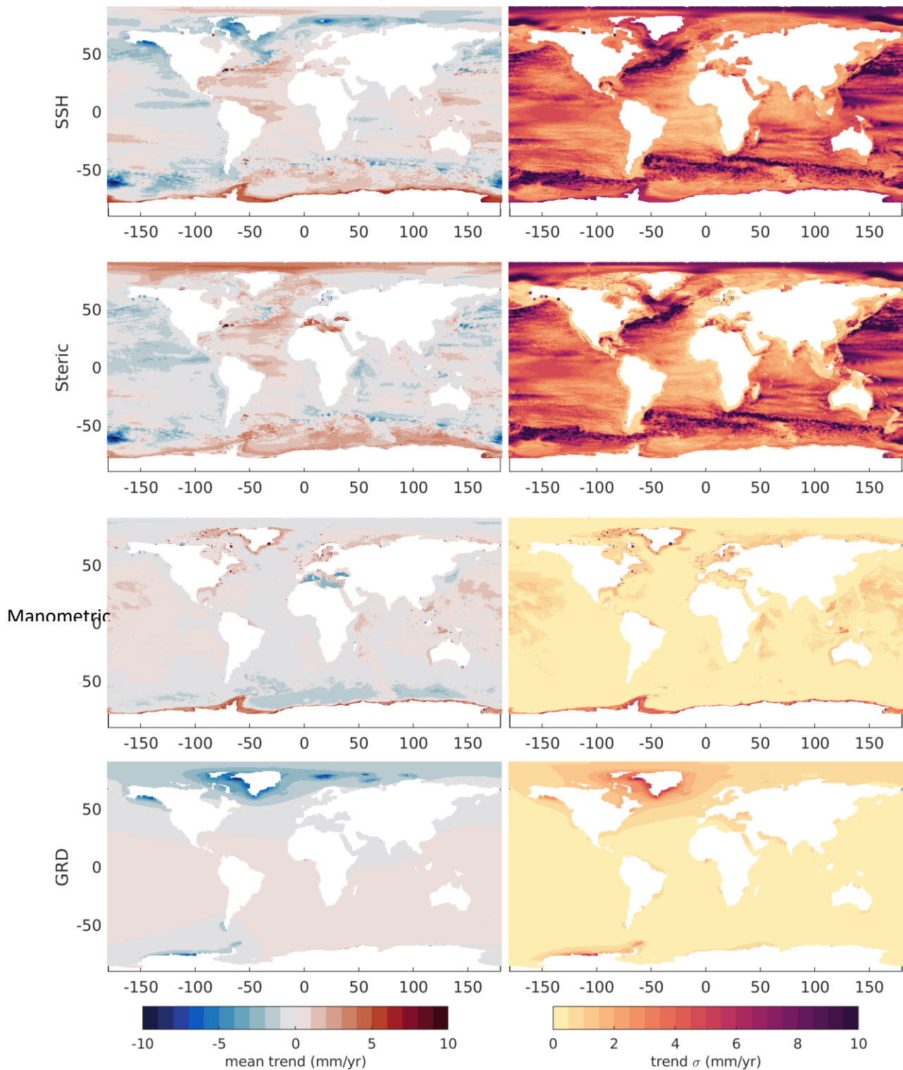
Figure S2. The time-mean (left) and standard deviation (right) of rolling, linear, decadal trends from the full NEMO model run, for SSH (top row), steric sea level (second row), dynamic manometric sea level (third row), and the gravitational, rotational and solid-Earth deformation (GRD) spatial redistribution (Frederikse et al., 2020) (bottom row).
