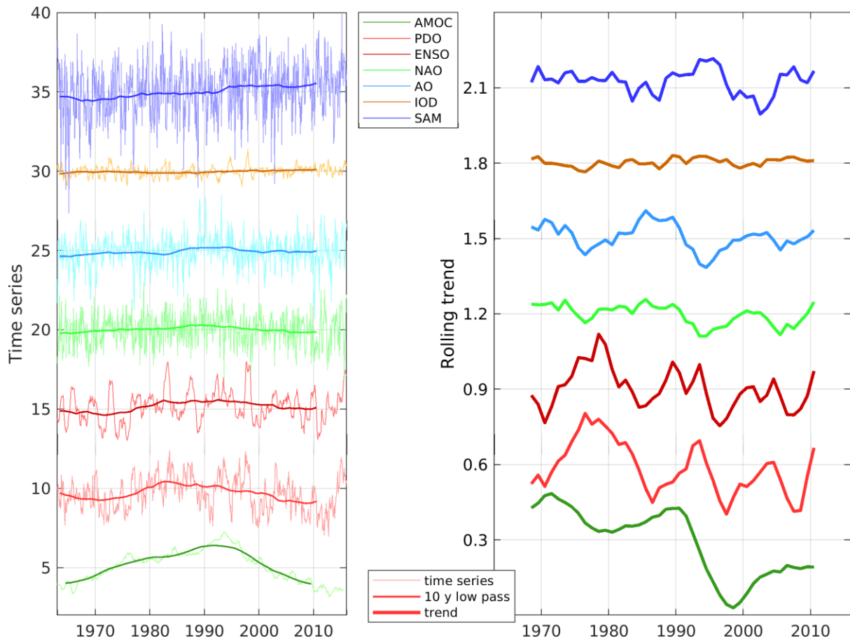
Figure S3. The time series (left) and decadal trends (right) of leading climate indices used in this study (see main text for the data citations).
