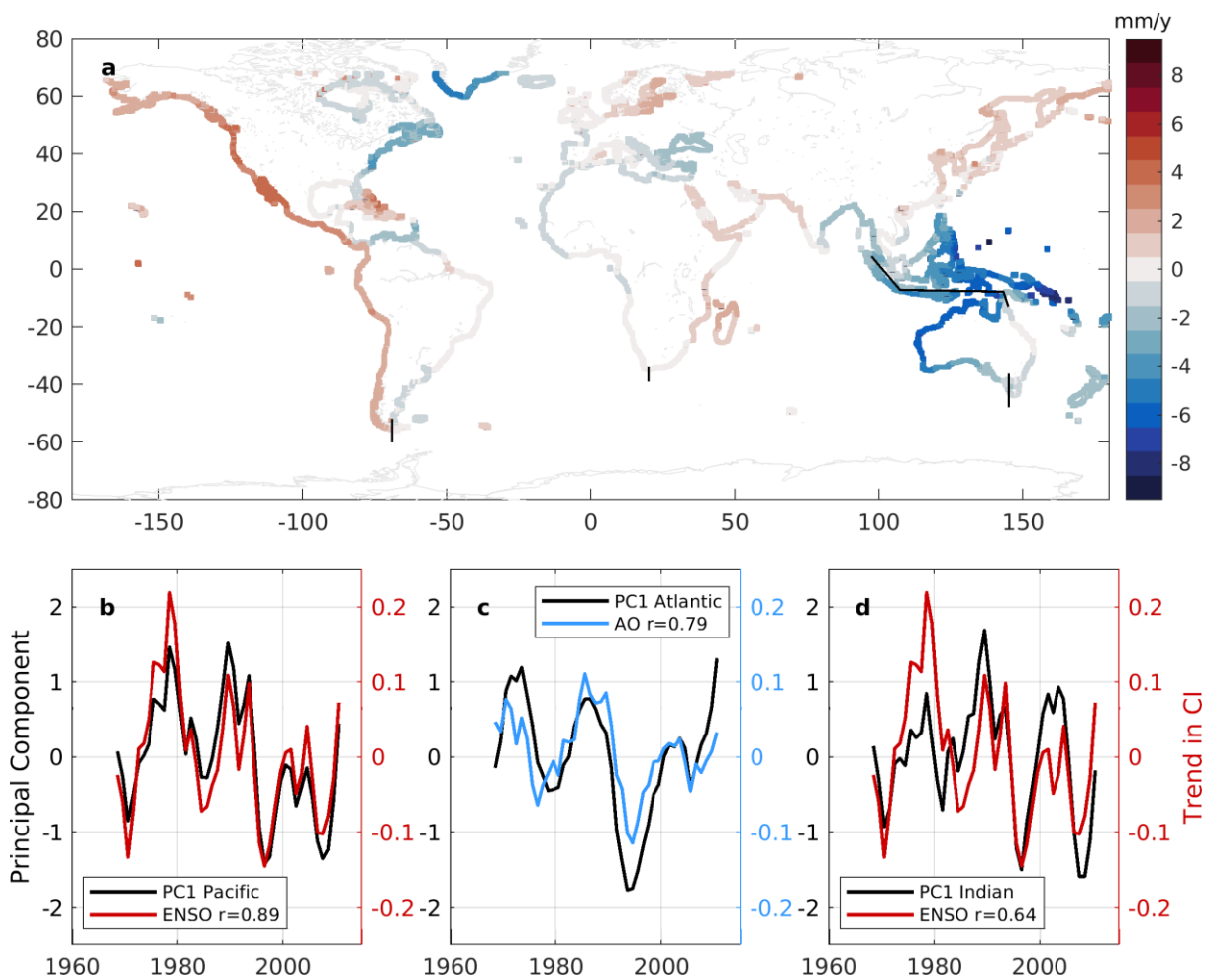
Figure S4. The spatial pattern (a) and rolling decadal trend PC1 for the Pacific (b), Atlantic (c), and Indian (d) Ocean basins shown with the climate index with highest correlation, for SSH.
