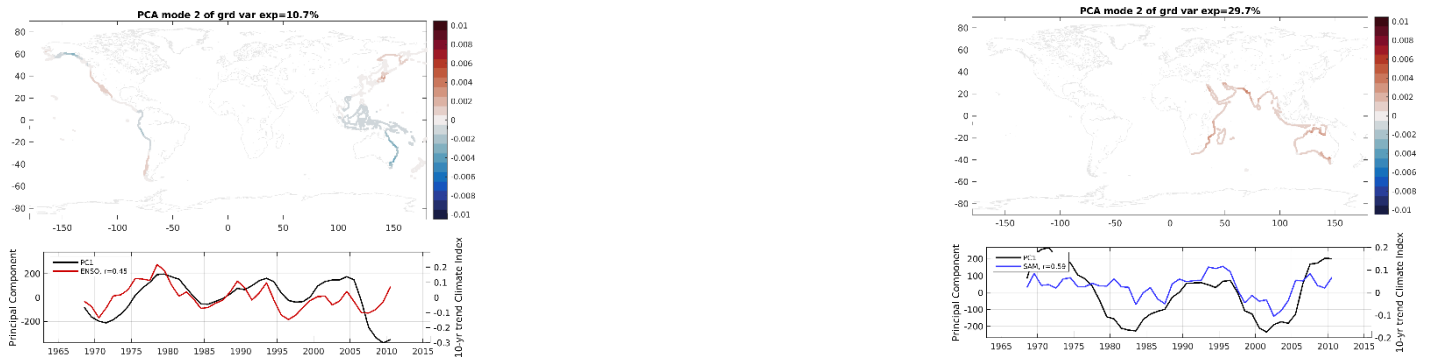
Figure S17. GRD PC2 spatial pattern (top) and rolling decadal trend (bottom). This pattern is ignored in the Atlantic basin in the reconstruction.
