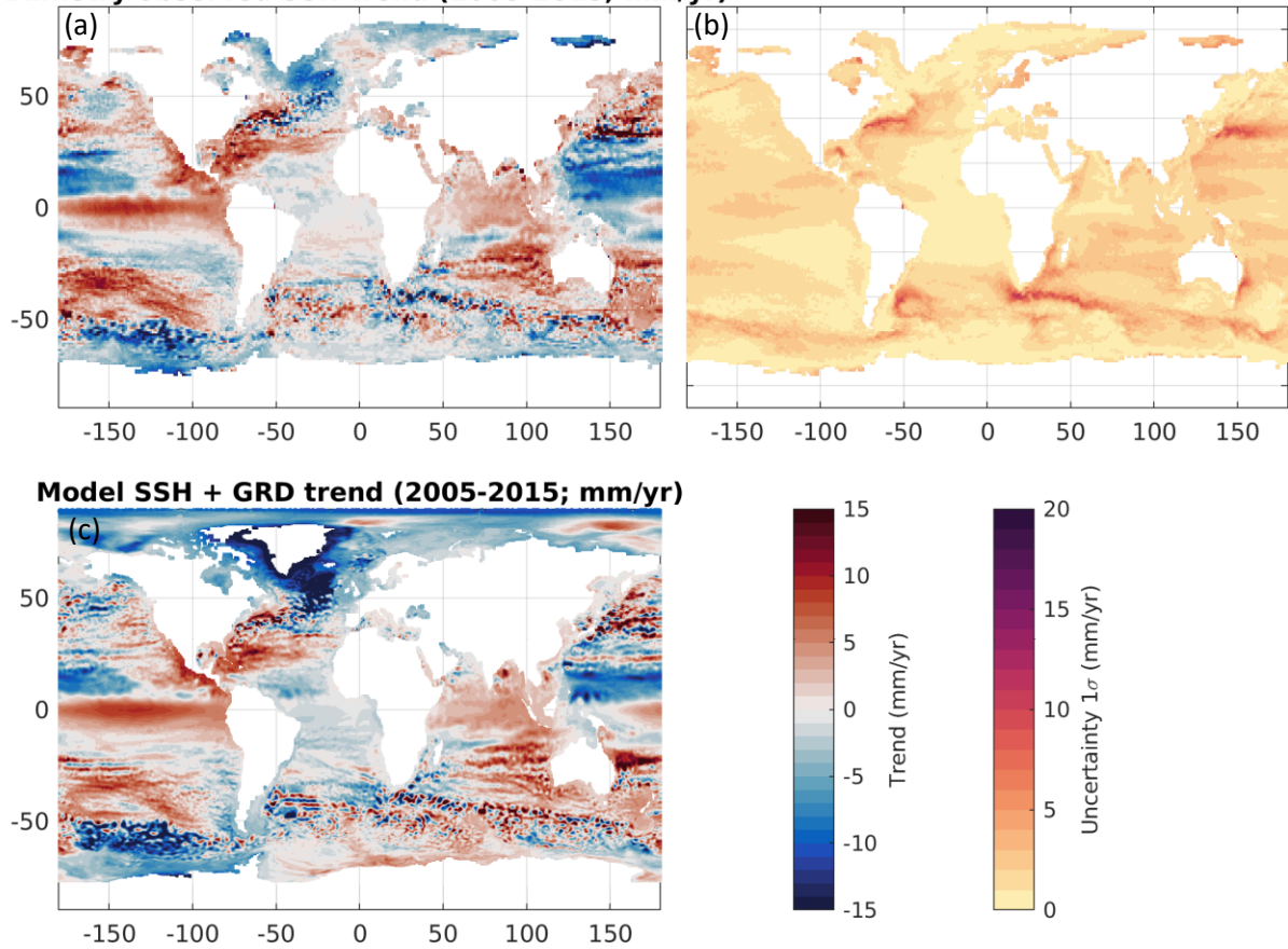
Figure S1. The linear trend from 2005—2015 inclusive for satellite altimetry observations (ESA SLCCI v2, ESA 2018) the decadal trend (a) and its uncertainty assuming an auto-regressive lag-1 noise (b) and the NEMO model plus GRD geoid spatial redistribution (Frederikse et al., 2020) (c).
