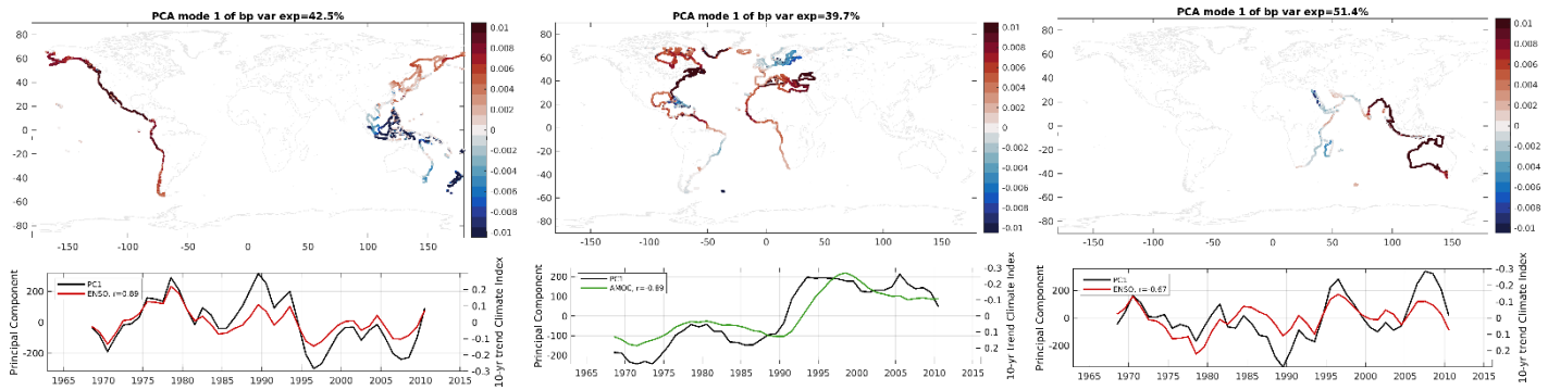
Figure S11. Manometric PC1 spatial pattern (top) and rolling decadal trend (bottom).
