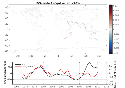
Figure S18. GRD PC3 spatial pattern (top) and rolling decadal trend (bottom). This pattern is ignored in the Atlantic and Pacific basins in the reconstruction.
