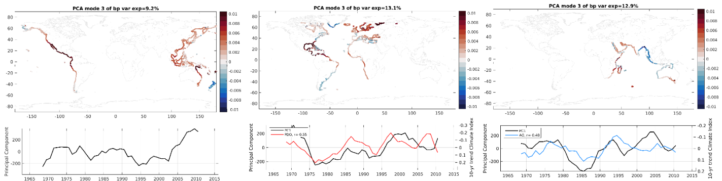
Figure S13. Manometric PC3 spatial pattern (top) and rolling decadal trend (bottom). This pattern is ignored in the Pacific basin in the reconstruction.
