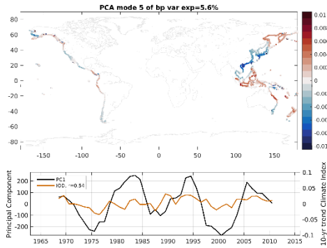
Figure S15. Manometric PC5 spatial pattern (top) and rolling decadal trend (bottom). This pattern is ignored in the Atlantic and Indian basins in the reconstruction.
