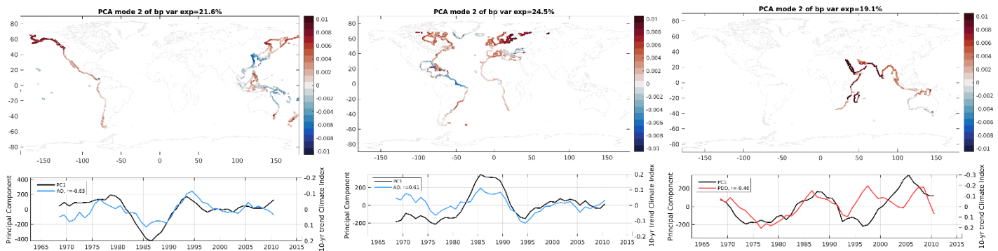
Figure S12. Manometric PC2 spatial pattern (top) and rolling decadal trend (bottom).
