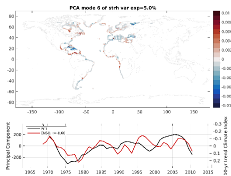
Figure S10. Steric PC6 spatial pattern (top) and rolling decadal trend (bottom). This pattern is ignored in the Pacific and Indian basins in the reconstruction.
