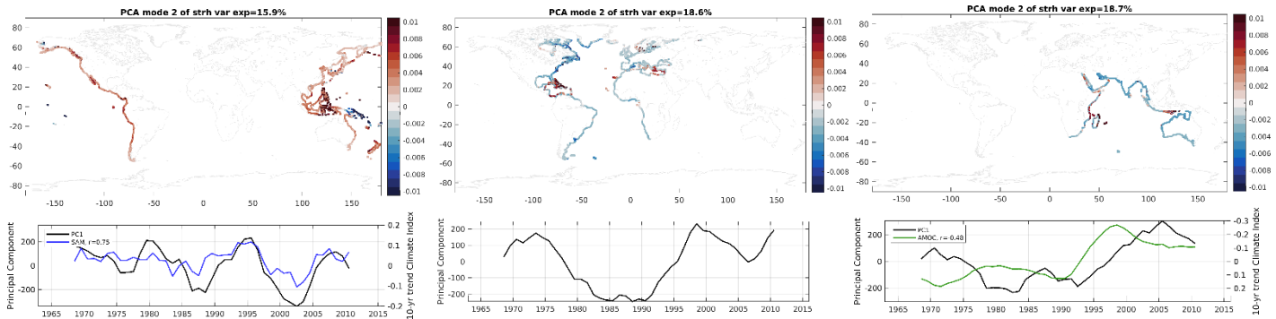
Figure S6. Steric PC2 spatial pattern (top) and rolling decadal trend (bottom). This pattern is ignored in the Atlantic basin in the reconstruction.
