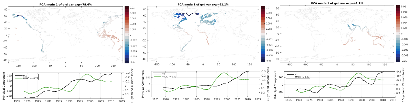
Figure S16. GRD PC1 spatial pattern (top) and rolling decadal trend (bottom).
