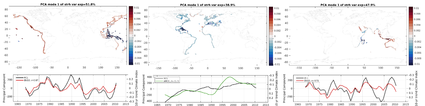
Figure S5. Steric PC1 spatial pattern (top) and rolling decadal trend (bottom).
