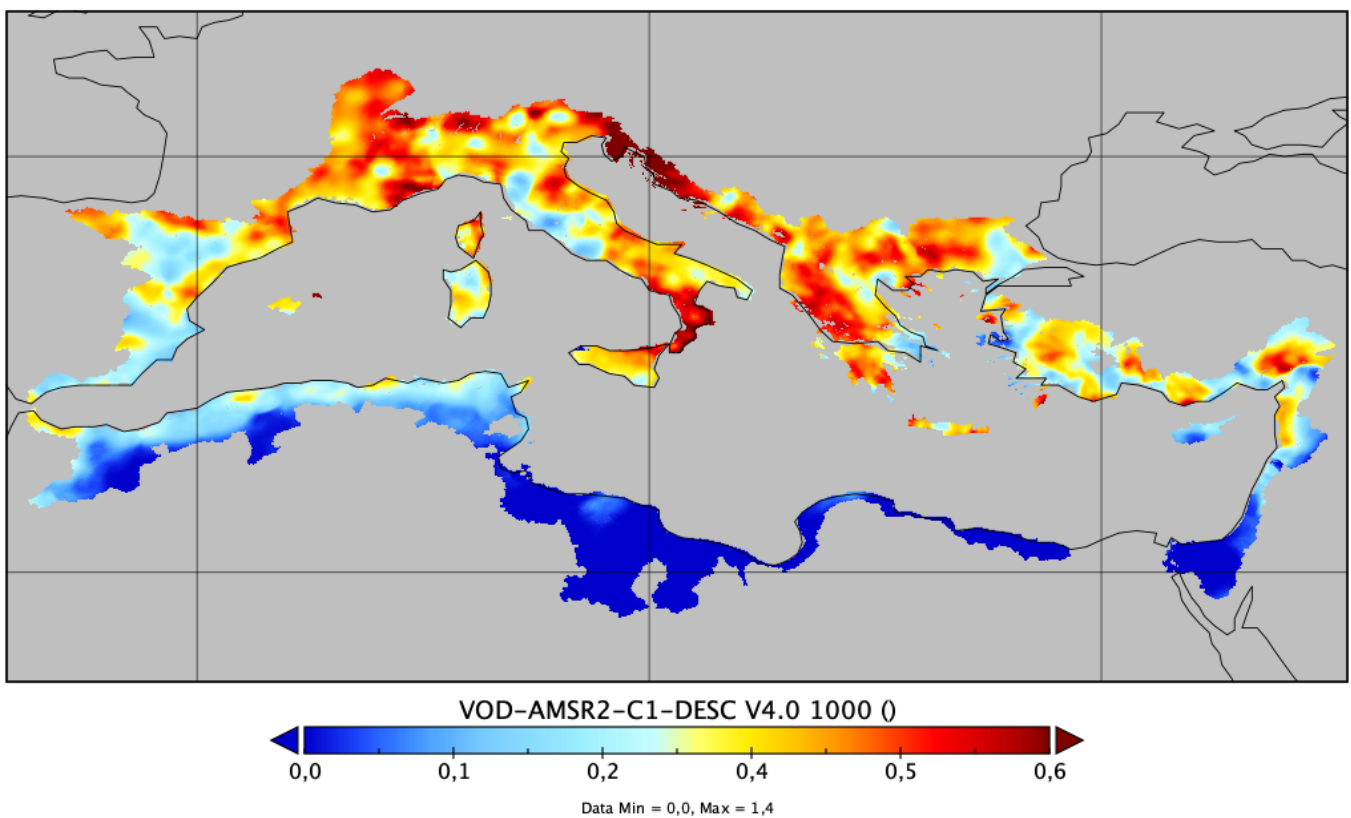
Figure 1: Average VOD for 2015 (C1 band) over the 4dmed spatial domain
