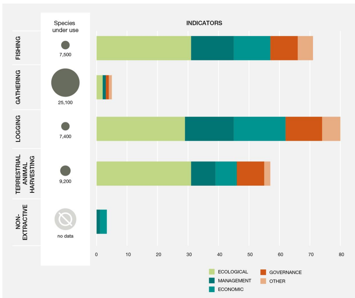
Figure SPM.6. Wild species used worldwide compared with indicators of sustainable use by practice. This figure displays the approximate number of wild species used, categorized by practice type, in comparison with the number of widely used global indicators of sustainable use of wild species by practice type. The terrestrial animal harvesting group is based primarily on a large regional indicator set due to the paucity of global indicators. Data for this analysis are from chapter 2 {2.3.2.2.2} and chapter 3 {3.2.1, table 3.1 and box 3.1 in 3.2.2}. A data management report for this figure is available at https://doi.org/10.5281/zenodo.6452576 .
