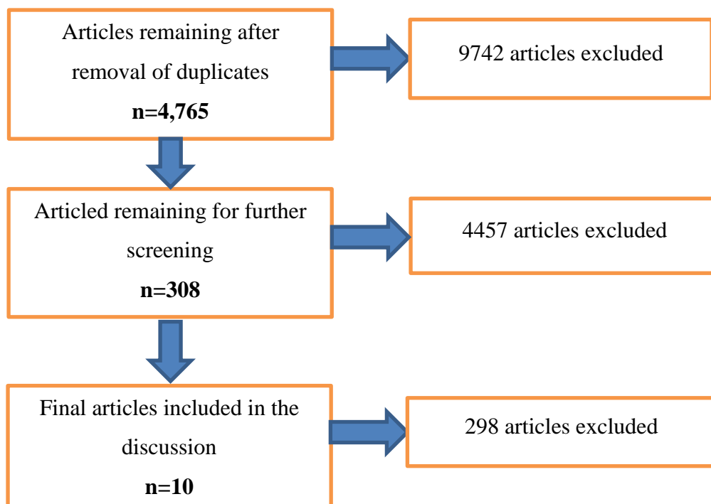
Figure 1: The flowchart
