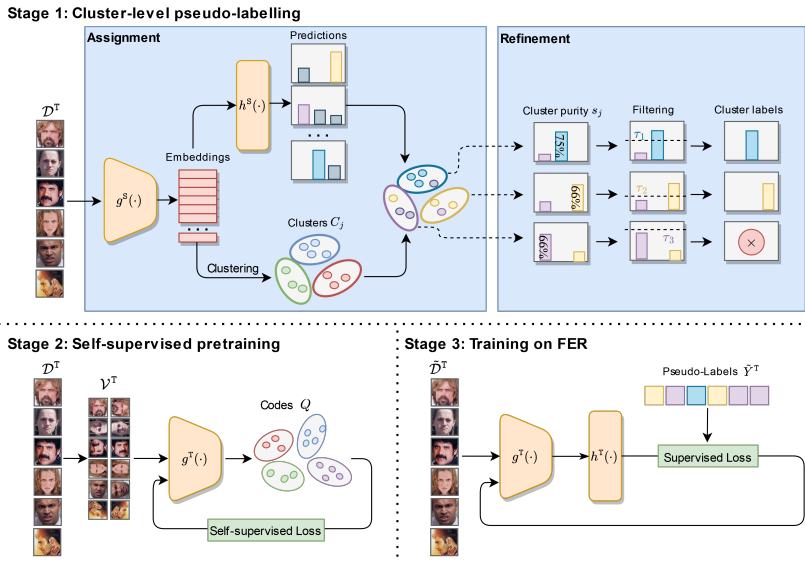
Figure 2: Our proposed CluP comprises of three-stage training, where the first stage produces trustworthy cluster-level pseudo-labels using the source model, the second stage warms up the target model in a self-supervised fashion, and finally the third stage performs the target model training with the refined pseudo-labels.
