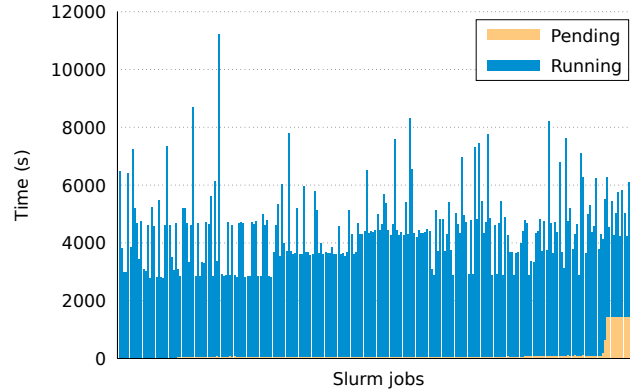
Figure 6.4: Execution times for the 240 DenseNet training experiments running in parallel on 240 GPU-equipped nodes of the CINECA MARCONI 100 facility.
