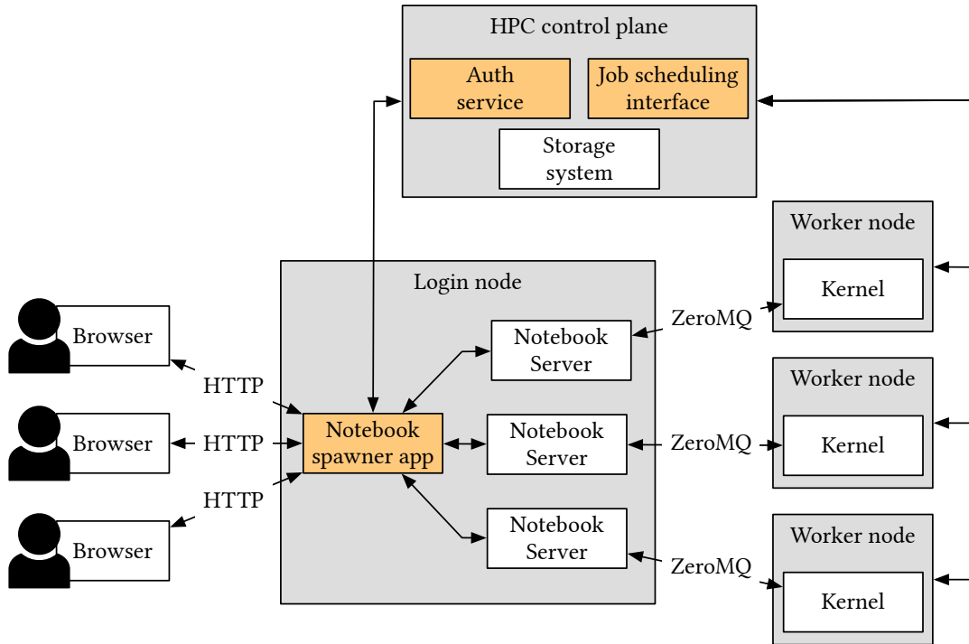
Figure 2.2: Sketch of the common architecture of a HPC Jupyter interface. Orange blocks usually need to be developed or extended to integrate Jupyter in the existing software stack.
