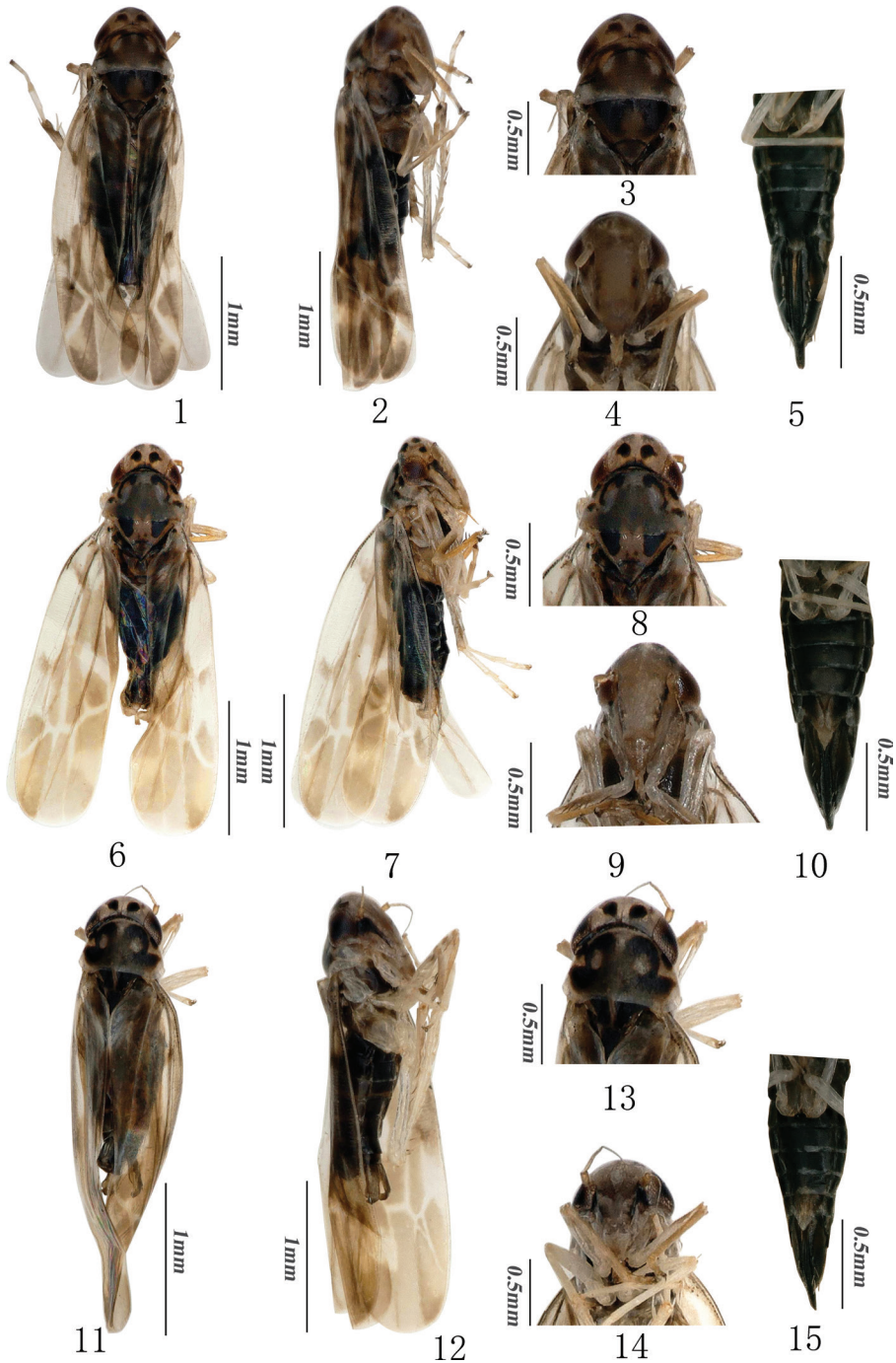
Figures 1–15. External morphology of Mitjaevia species 1–5 Mitjaevia bijiensis sp. nov. 1 habitus, dorsal view 2 habitus, lateral view 3 head and thorax, dorsal view 4 face 5 female thorax and abdomen, ventral view 6–10 Mitjaevia solitaria sp. nov. 6 habitus, dorsal view 7 habitus, lateral view 8 head and thorax, dorsal view 9 face 10 female thorax and abdomen ventral view 11–15 Mitjaevia salaxia sp. nov. 11 habitus, dorsal view 12 habitus, lateral view 13 head and thorax, dorsal view 14 face 15 female thorax and abdomen, ventral view.
