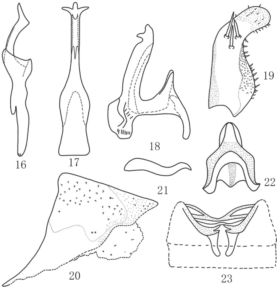
Figures 16–23. Mitjaevia bijiensis sp. nov. 16 style 17 aedeagus, ventral view 18 aedeagus, lateral view 19 subgenital plate 20 male pygofer, lateral view 21 pygofer dorsal appendage, lateral view 22 connective 23 abdominal apodemes.
