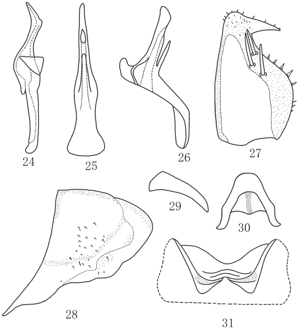
Figures 24–31. Mitjaevia solitaria sp. nov. 24 style 25 aedeagus, ventral view 26 aedeagus, lateral view 27 subgenital plate 28 male pygofer, lateral view 29 pygofer dorsal appendage, lateral view 30 connective 31 abdominal apodemes.
