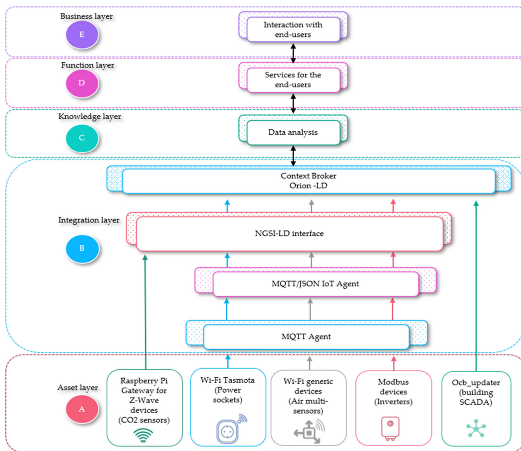
Figure 4. Implementation of PHOENIX architecture in PoC.
