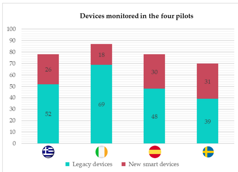
Figure 6. Integrated devices from the four pilots.
