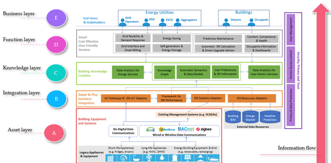
Figure 2. PHOENIX-architecture diagram.
