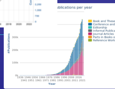
DBLP statistics
