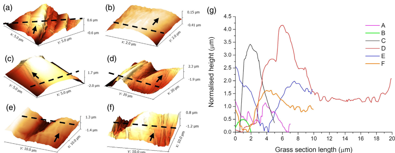
FIGURE 2 (a to f) 3D AFM images of decellularized grass and the corresponding topographic height plots (g) normalized to the minimum z -axis data point. Arrows = longitudinal direction of grass blade. Black dotted line = specific cross-section mapped onto the height plot
