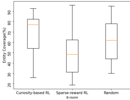
Figure 4: Per episode entity coverage on 8-room level
