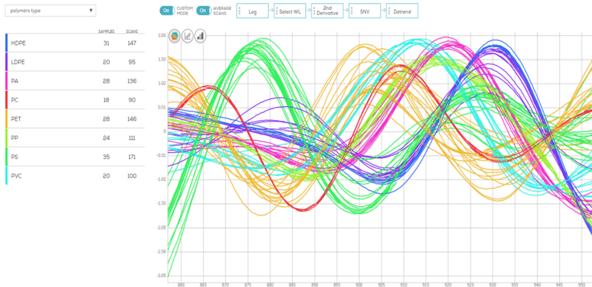
Figure 17 Spectra from the polymers after data treatment (log, average, 2 nd derivative) from the selected wavelength range of 850-950 nm.
