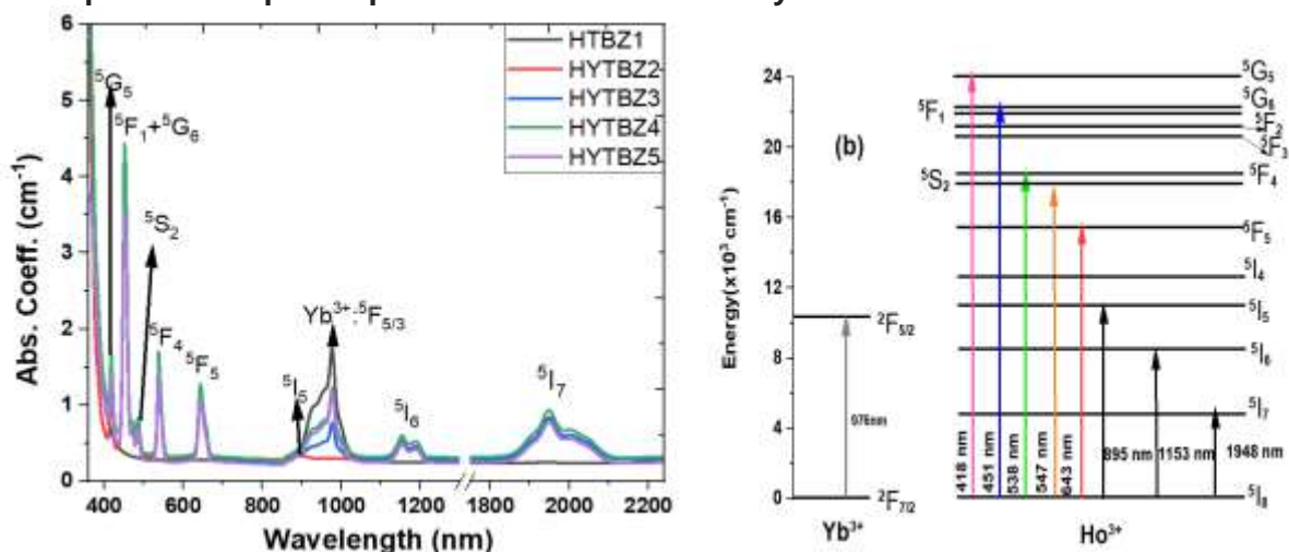
Fig. 2: (a) UV-visible-NIR absorption coefficient spectra of Yb 3+ , Ho 3+ single doped and Ho 3+ -Yb 3+ codoped barium fluorotellurite glass series, (b) Partial energy level diagram of Ho 3+ ion.
