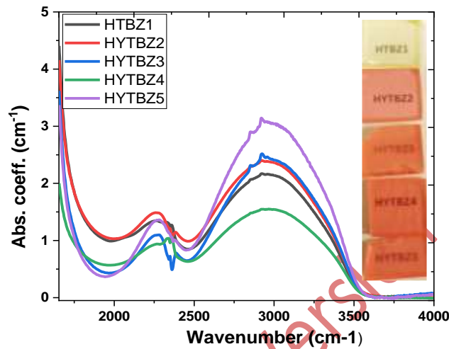
Figure 1: Infrared absorption spectra of singly Yb 3+ , Ho 3+ doped, and Ho 3+ :Yb 3+ codoped fluorotellurite glasses and the inset showing photographs of various glasses prepared.
