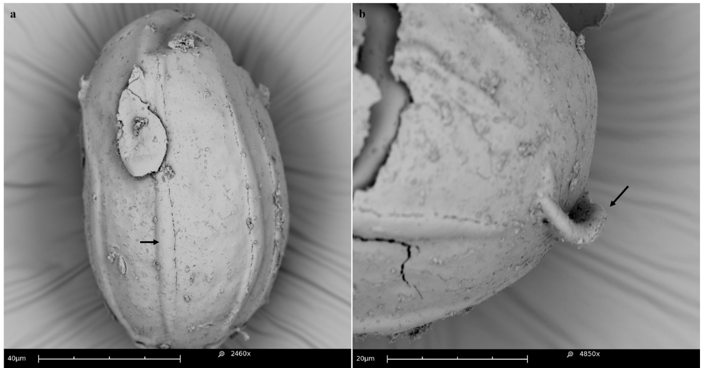
Figure 2 External morphology of the B. yothersi eggs: (a) – transverse streaks or carinae (arrow) and (b) – fold-like structure (arrow). Scale bar length (a) 40 μm and (b) 20 μm.
