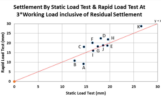
Figure 7- Settlement comparison between Static test and Rapid Test at 3 x Working Load with residual settlement accounted
