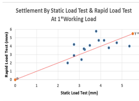
Figure 5- Settlement comparison between Static test and Rapid Test at 1x Working Load.
