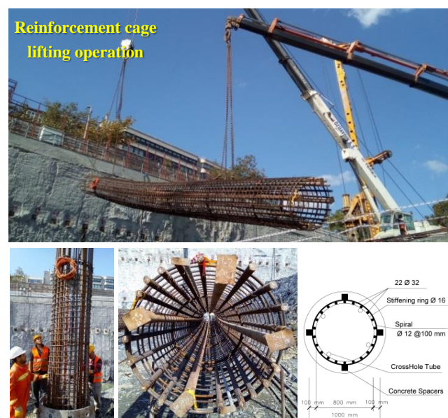
Fig. 2. General views from the pile installation and reinforcement cage detail.
