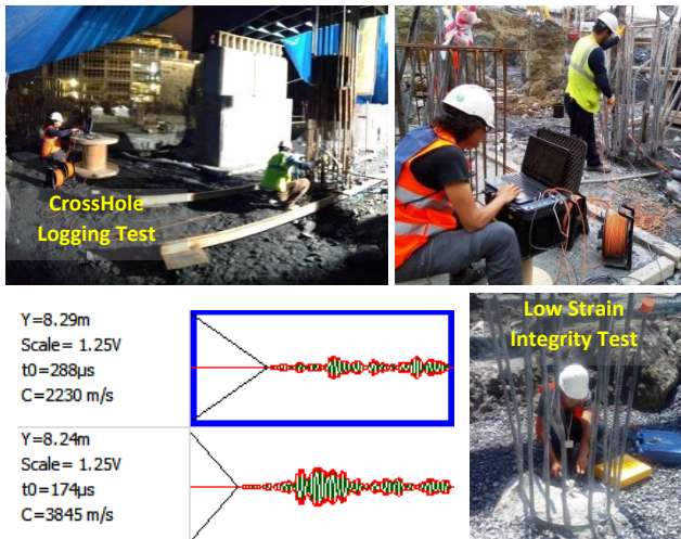
Fig. 8. General views from low strain integrity and crosshole logging test.
