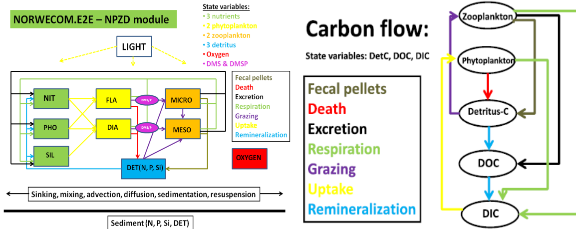
Figure 4. Schematics of the NORWECOM.E2E NPZD module (left) and the carbon flow (right)
