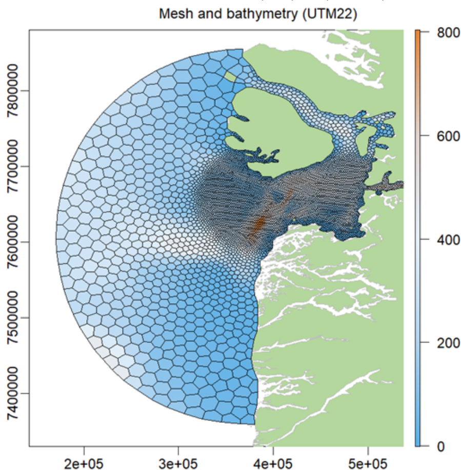
Figure 11. Computational mesh (polygons) and bathymetry for the Disko Bay area. Bathymetry is interpolated from the IceBridge BedMachine Greenland (Version 3) bathymetry and shown in colors.
