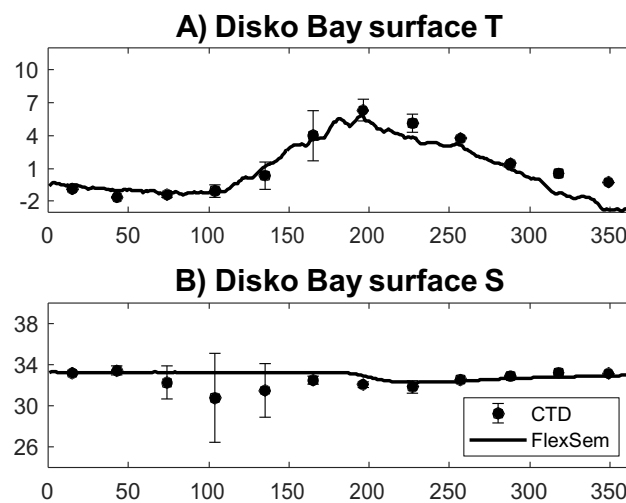
Figure 13. Time-series of A) surface temperature and B) salinity during from CTD data (means±SD: 1992-2012) and FlexSem (2004) from a station near Qeqertarsuaq south of Disko Island.
