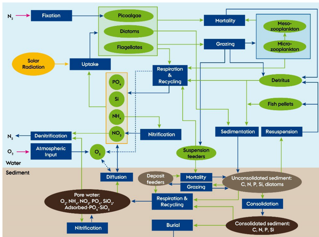
Figure 12. Model diagram showing the pelagic (green circles) and benthic (brown circles) state variables and associated fluxes (blue boxes) in the ERGOM model. The model diagram was modified from Maar et al. (2018) by exchanging cyanobacteria with picoalgae.
