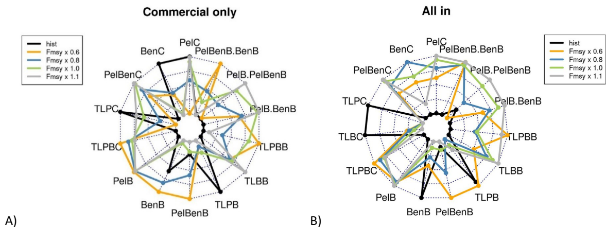
Figure 9. Indicators calculated for the historical time slice (2005-2015, in black), and for the future time slice (2055-2065) for the four scenarios. In A) the results from the scenarios only including the currently harvested species are displayed, while B) a show the scenarios including harvest on e.g., meso-zooplankton and meso-pelagic fish. The historical time slice is equal across all simulations. Indicators are all shown with maximum (best) value at the outer edge of the spider plot. The indicators shown include catches (C) and biomass (B) for the functional groups (Pel - pelagic, Ben - Benthic and PelBen - benthic-pelagic) and for the trophic levels (TL).
