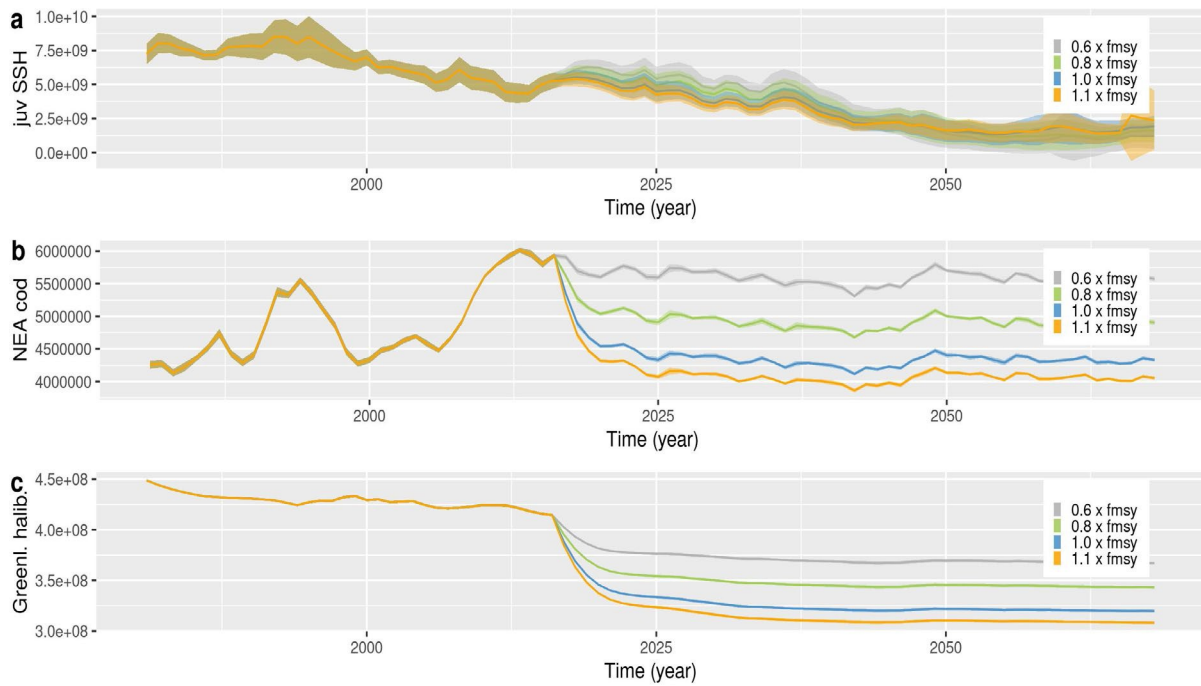
Figure 8. Simple indices for juvenile herring (a), northeast Atlantic cod (b) and Greenland halibut (c) for the period from 1981-2068. Shades represents one standard deviation across the 14 replicates of each scenario, whereas the solid line is the average across the simulations. Figure from Hansen et al., 2021.
