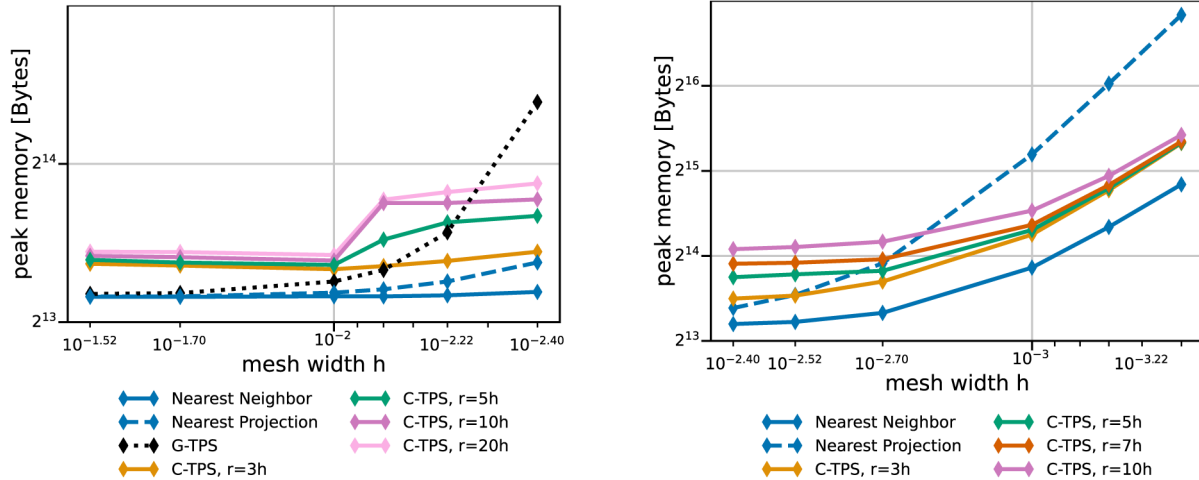
Figure 11. Comparison of the maximum overall memory consumption of various data mapping methods for coarse series (left) and fine series (right) from Table 2. Participant S_1 uses h = 0.009 for the coarse series (left) and h = 0.0014 for the fine series (right). The memory consumption is the maximum of all ranks of participant S_2 , which is executing the mapping.
