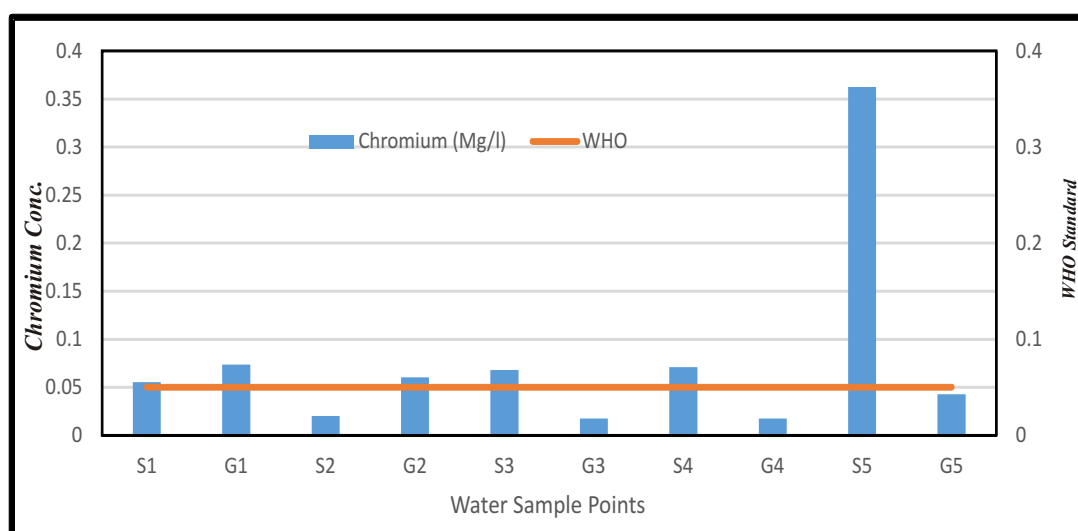
Figure 4: Concentration of chromium in surface and ground water at BBL, Makurdi
