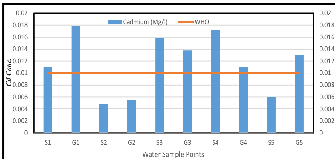
Figure 2: Concentration of cadmium in surface and ground water at BBI, Makurdi
