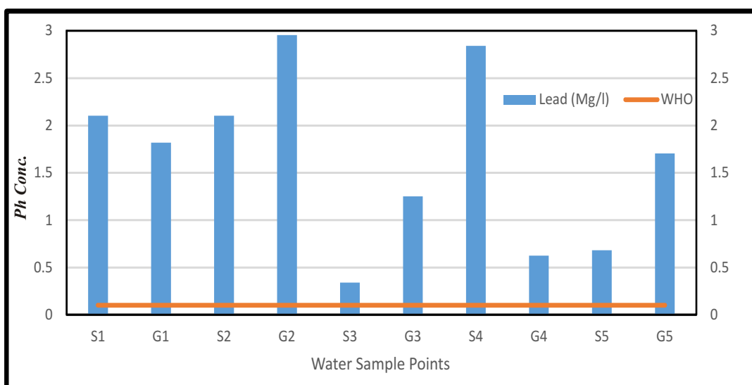
Figure 3: Concentration of lead in surface and ground water at BBI, Makurdi
