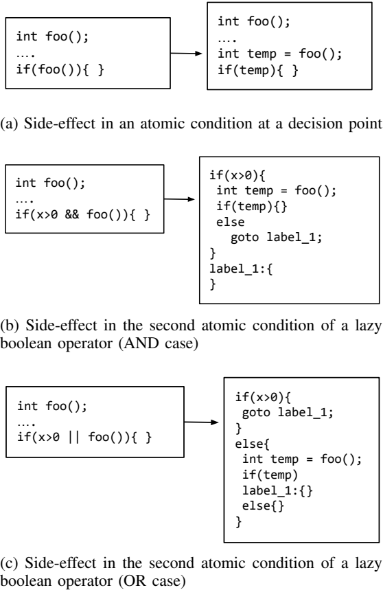
Fig. 6: Extracting side-effects from atomic conditions at program decision points.
