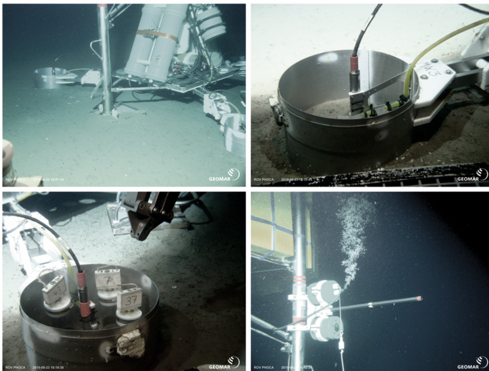
Fig. 3: Sampling of the arcFOCE experiment during RV Polarstern expedition PS121: experimental setup at 1500 m water depth off Svalbard (top left), close-up of one of the mesocosms perfectly in place at the seafloor (top right), sediment sampling inside a mesocosms using ROV-handled push-corers (bottom left), blowing off excess CO 2 before recovering the bottom-lander (copyright: GEOMAR).
