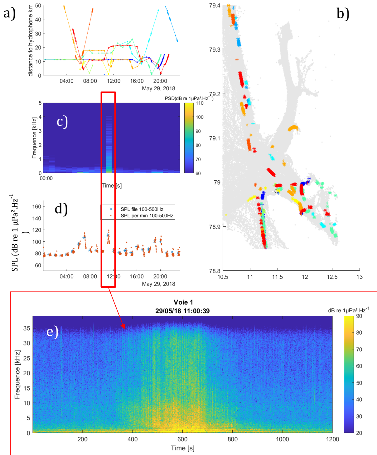
Fig. 8: Comparison of boats activity, i.e. distance from hydrophone (a) and AIS position (b), with acoustics measures, i.e. spectrogram (c) and SPL (d), among one day of recording. Example of a boat passage around 11:10 am with a decrease of distance from the hydrophone in a) and an increase of intensity on c), d) and zoomed in e) (acoustic signature at 600 s of the spectrogram).
