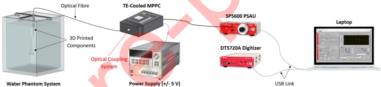
Figure 3. Schematic diagram of the TE-cooled SiPM + full optical coupling system experimental set-up.
