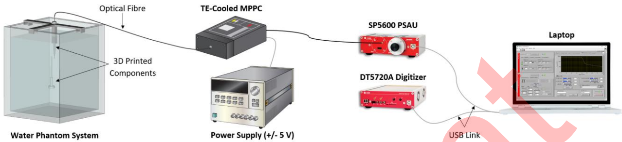
Figure 2. Schematic diagram of the TE-cooled SiPM experimental set-up.
