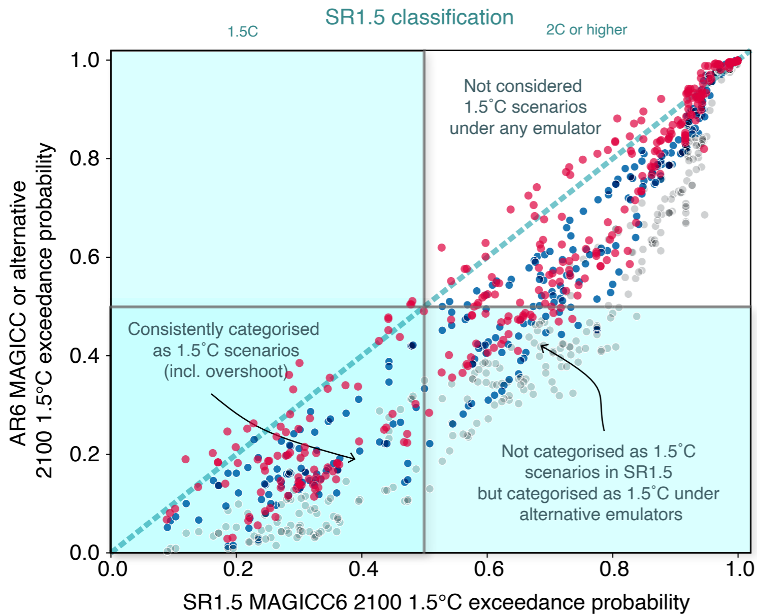
a 2100 exceedance probability of 1.5°C
