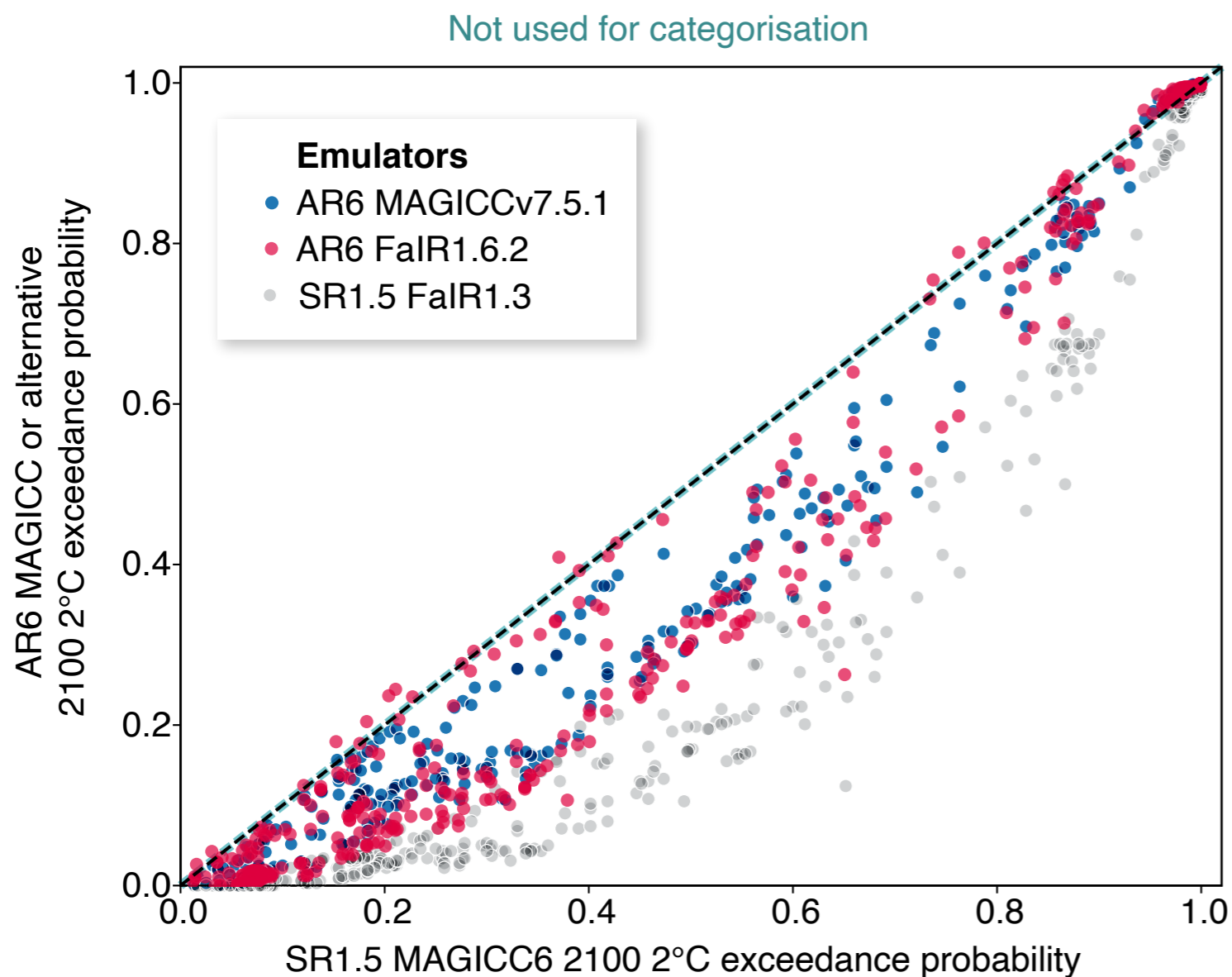
c 2100 exceedance probability of 2°C
