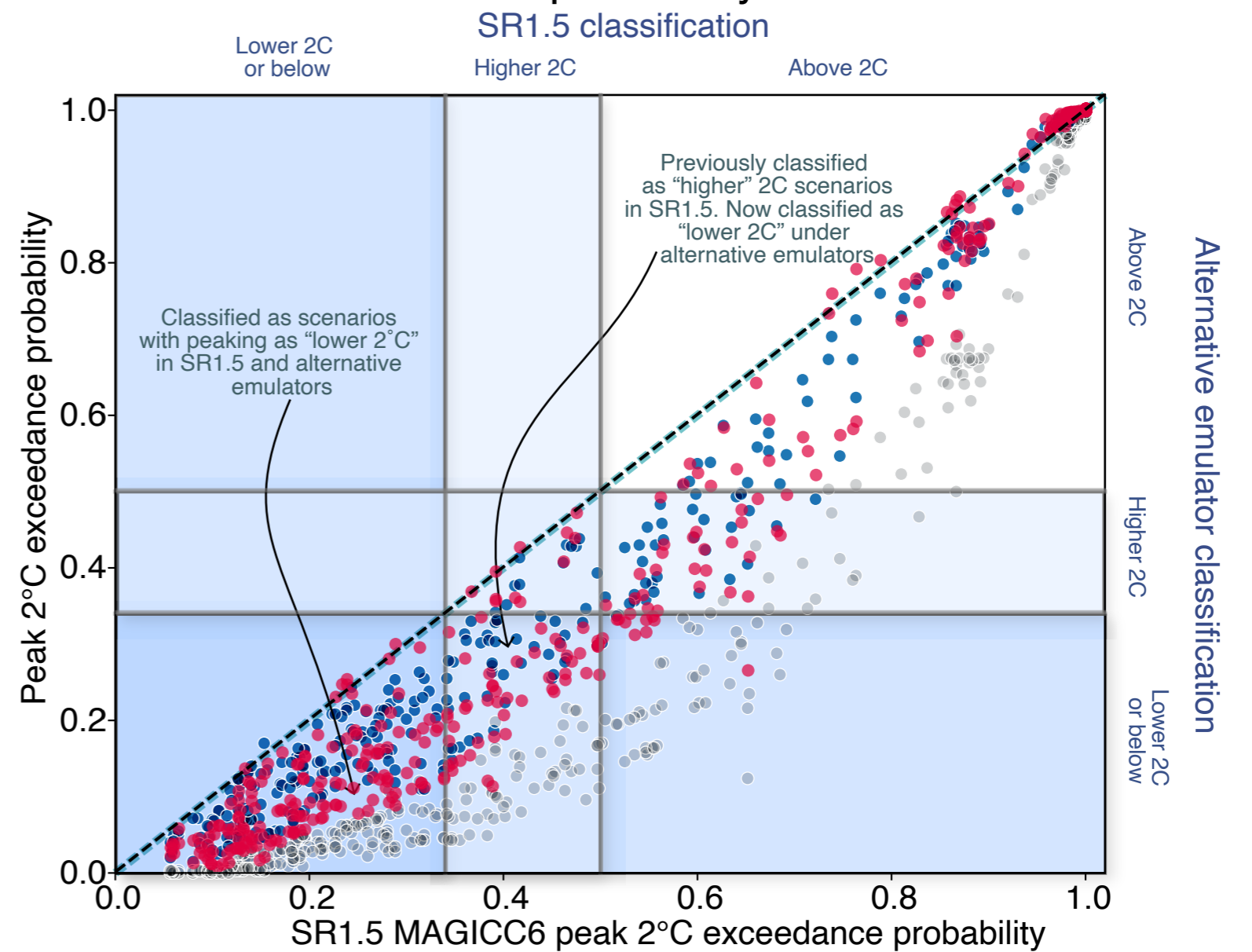
d Peak exceedance probability of 2°C
