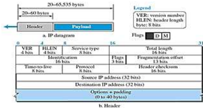
Figure 2. IP datagram
