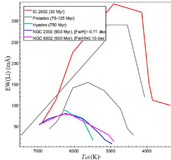
Figure 3.29: EW(\text{Li}) -versus- T_{\text{eff}} diagram comparing the upper Li envelopes for NGC 2355 (900 Myr, [\text{Fe}/\text{H}]=-0.11 dex) and NGC 6802 (900 Myr, [\text{Fe}/\text{H}]=0.10 dex).
