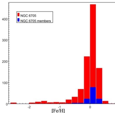
5) [Fe/H] metallicity
