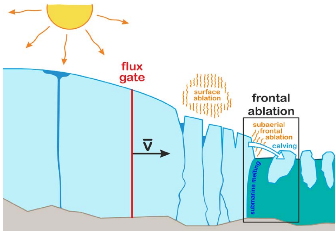
Figure 11. Illustration of mass loss from a glacier resulting icebergs drifting in the ocean.
