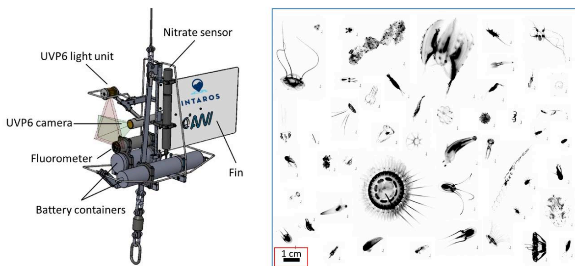
Figure 16. Left: Sensor package setup with an Underwater Vision Profiler 6 (UVP 6), which acquires particle sizes and quantities as well as zooplankton and aggregate images. The fluorometric SUNA sensor measures nitrate concentrations, the Ecotriplet sensor acquires chlorophyll-a, cDOM, and particle backscatter. Right: example of image showing of Arctic zooplankton from the location north of Svalbard. Figures are provided by A. Rogge, AWI.
