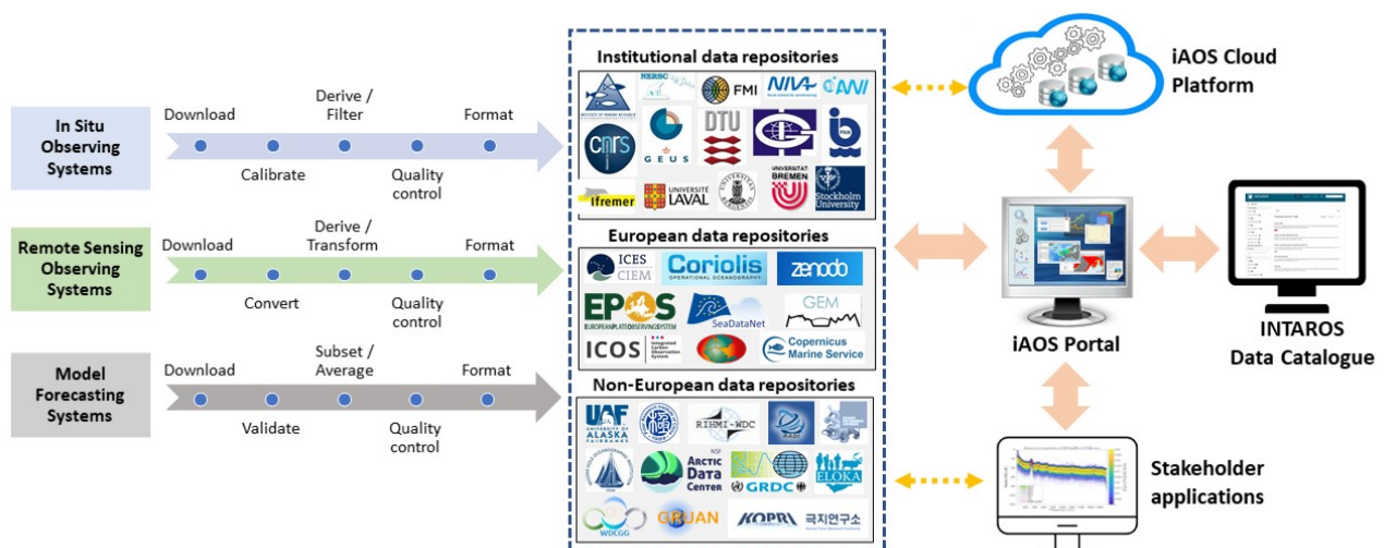
Figure 4. Data delivery chains focused for integrating INTAROS data into the various iAOS subsystems (portal, data catalogue, cloud platform, stakeholder applications).
