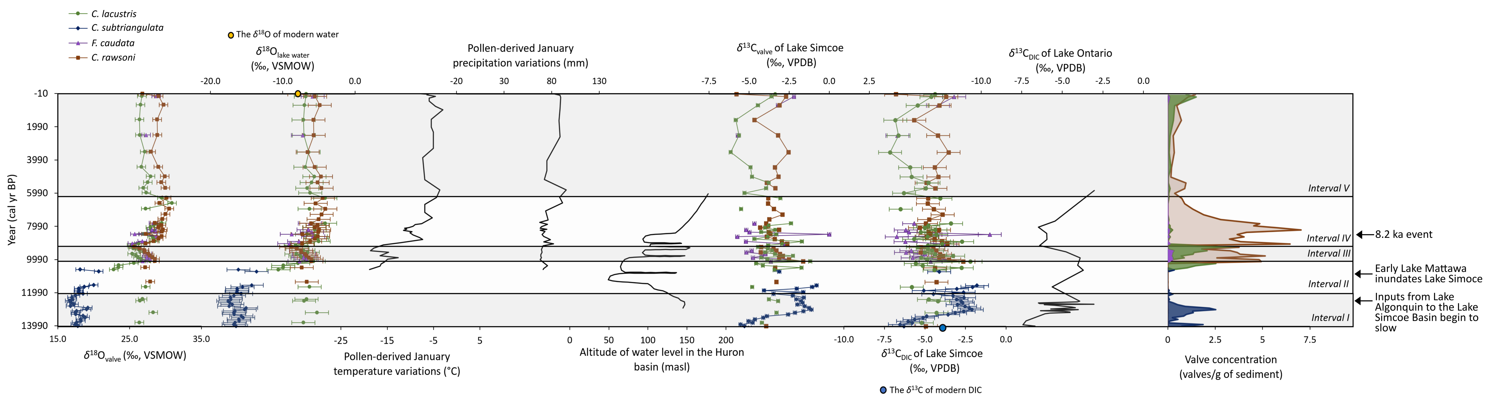
Figure 3. Proxies derived from ostracods in core PC-5 from Lake Simcoe compared with previously published records. January temperature and precipitation reconstructions are derived from pollen assemblages in PC-5 (Volik et al., 2016). The altitude of water level in the Huron Basin was first reported in Lewis et al. (2005, 2012). The \delta^{13}C_{\text{DIC}} from Lake Ontario was first reported in Hladyniuk and Longstaffe (2015).
