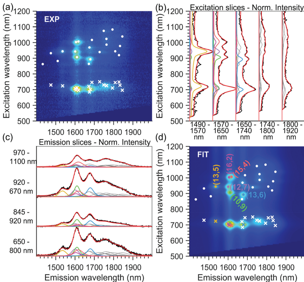
Fig. 4 Example PLE map and fit for the T_{4T_3} sample: (a) experimental PLE map cut to the desired fitting range (b) normalized excitation and (c) emission slices obtained by integrating the PLE maps over certain emission and excitation ranges, respectively, as indicated on the bottom (panel b) or left (panel c) of each slice. Experimental data are plotted in black and fitted data in red. Moreover, we also show the contributions of the different chiral structures in the PLE fit. The contribution of the chiralities labelled in panel (d) are highlighted with the same colour, the contribution of the other chiralities are plotted in grey. (d) Fitted PLE map with overlaid fitted SWCNT peak positions (white and coloured dots) and fitted EET peak positions (white and coloured crosses).
