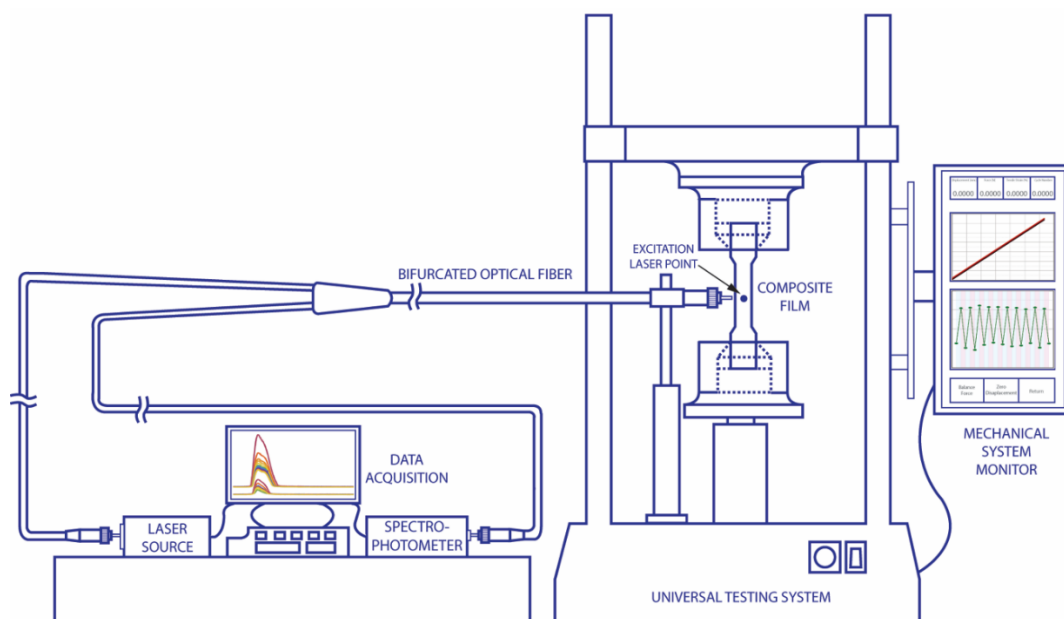
Figure S5. Customized set-up used for investigating in-situ the photoluminescence of the MHLP-PDMS free-standing films under mechanical cyclic stretching.
