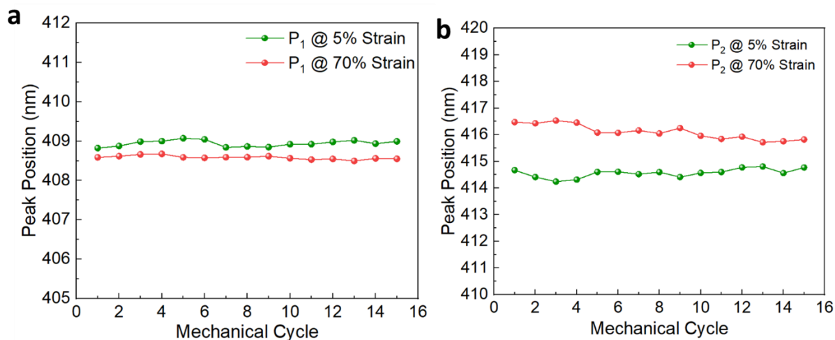
Figure S9. Position of the emission peaks P 1 and P 2 as a function of the number of stretch/release cycle applied to the (BzA) 2 PbBr 4 -PDMS free-standing films prepared with 2% in vol. of MHLP. A red-shift of less than 2 nm is observed on both peak while stretching the films up to 70% strain.
