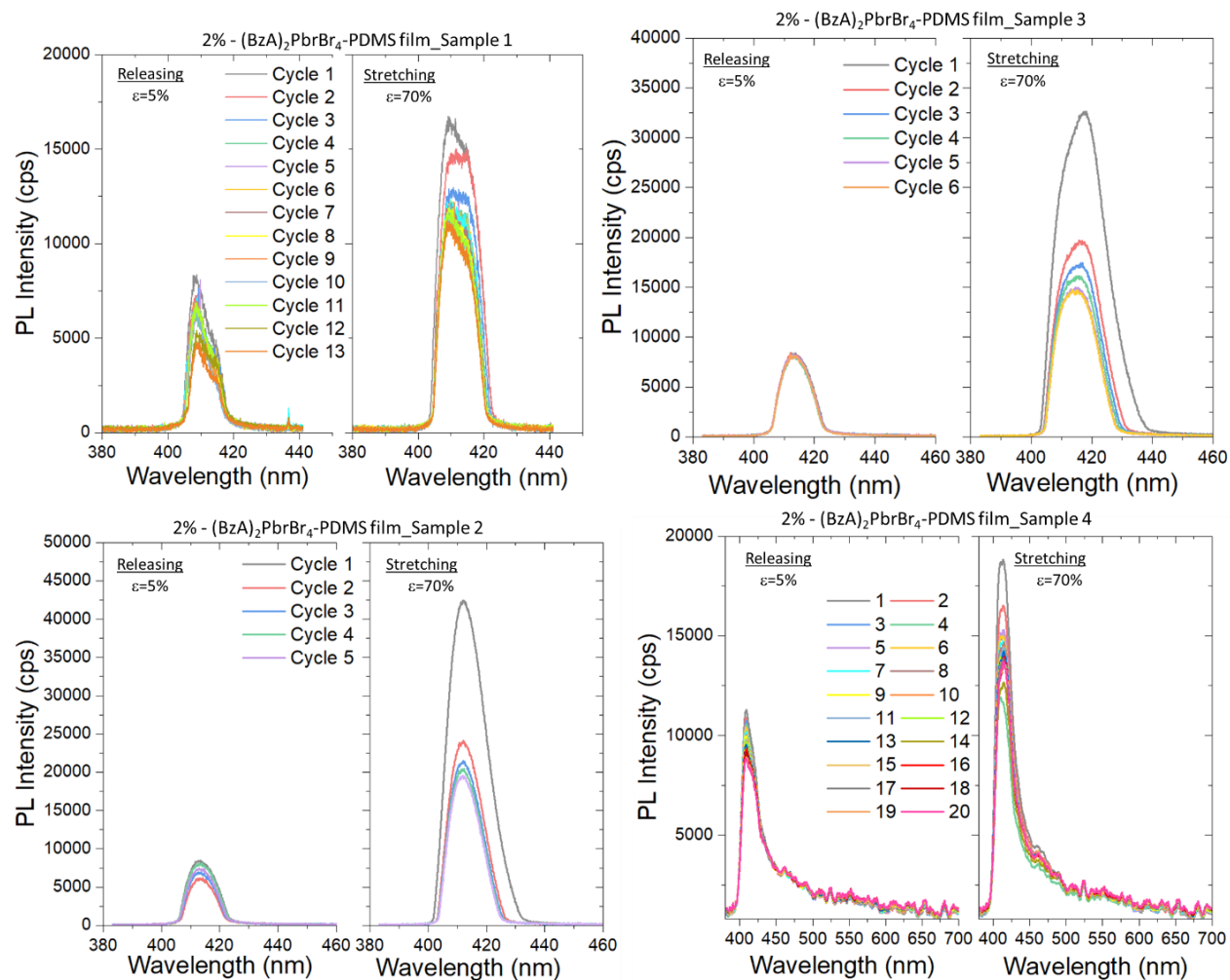
Figure S6. Emission spectra acquired from four different (\text{BzA})_2\text{PbBr}_4 -PDMS free-standing films prepared with 2% of perovskite precursors under continuous stretch/release mechanical cycles. All of them show around 1.5 (sample 4) to 2.5 fold increase in PL intensity after stretching.
