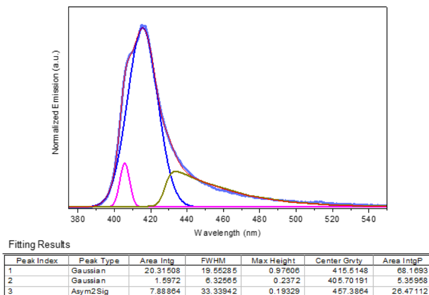
Figure S4. Results of the fitting PL profile of the MHLP-PDMS film, with an adjusted R-squared of 0.9991. The PL of the film and the resulting fitting curve are shown in blue and red, respectively. The two characteristic emission peaks are centered at 406 nm ( P_1 , in magenta) and 416 nm ( P_2 , in blue), with corresponding full width at high maxima (FWHM) of 6 nm and 20 nm.
