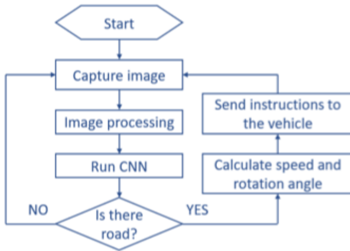
Fig. 26.1: Autonomous vehicle navigation algorithm workflow.
