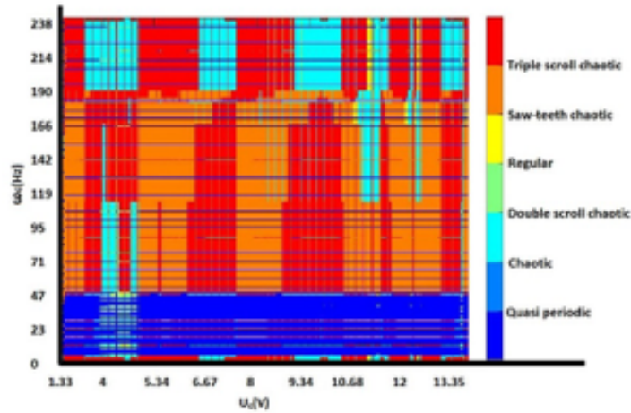
Fig. 35.8: The ANN dynamic classification graph on the plane of magnetic field strength equivalent to the applied voltage to the electromagnet and angular speed of rotor.
