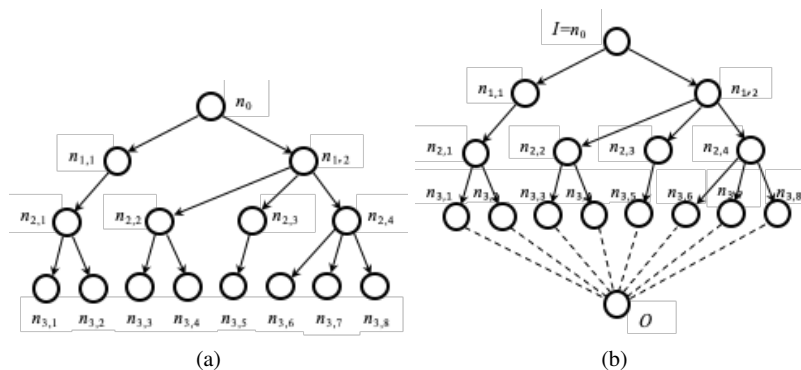
Fig. 37.3: (a) A tree data structure example. (b) A lattice results in by inserting an additional level including the least lattice element O . The tree root corresponds to the greatest lattice element I .
