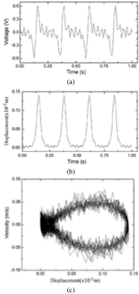
Fig. 35.5: Experimental data which is generated for 3.5 m/s wind speed.
