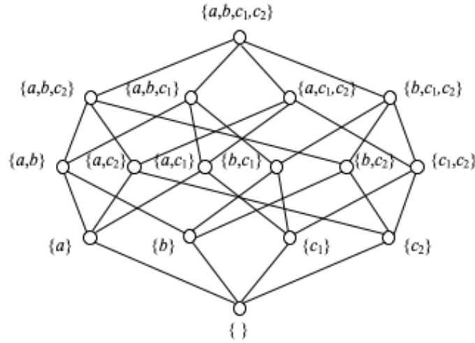
Fig. 37.4: A Boolean lattice ontology of the four inequality constraints a: TSS_{min} < TSS < TSS_{MAX} , b: T_{amin} < TA < T_{AMAX} , c1: pH < pH_{MAX} and c2: pH_{min} < pH , regarding grape maturity indices TSS, TA and pH.
