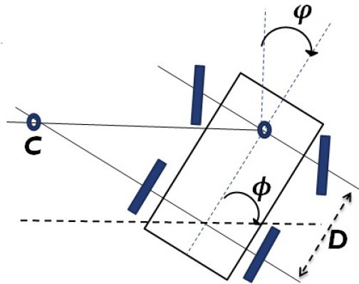
Fig. 17.1: Four wheel robot
