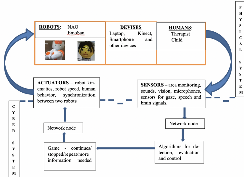
Fig. 38.2: Robot-based CPS for children with communication disorders with human in the loop
