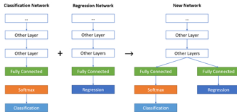
Fig. 26.4: New proposed network architecture.
