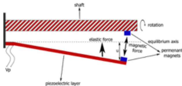
Fig. 35.2: The operation mechanism of the wind harvester under elastic and magnetic forces.
