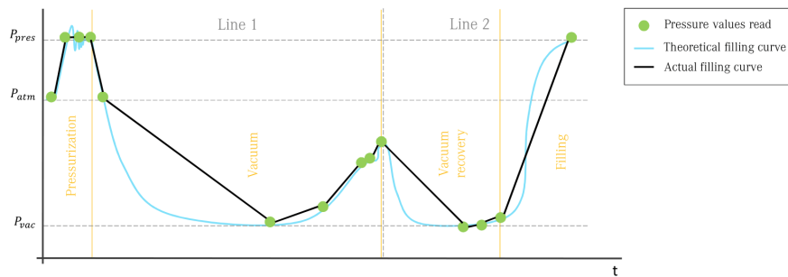
Fig. 29.1: Comparison between the theoretical and actual A/C filling curves that can be obtained through the data gathering mechanisms currently implemented on the process.
