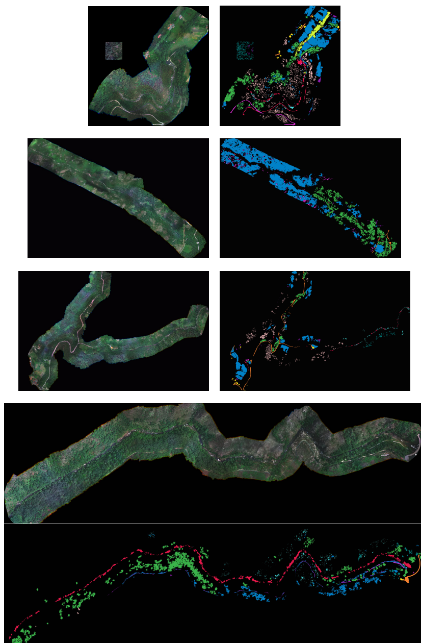
Fig. 8.4: Some of the multispectral datasets used in the experiments. Color composite and reference data for the Oitavén, Xesta, Eiras and Ermida datasets, respectively.
