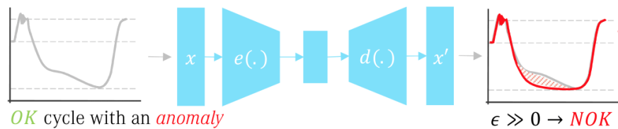
Fig. 29.3: The received cycle is marked as OK and it does contain an anomaly. This is perceived in the reconstruction error, making a warning signal to be raised.
