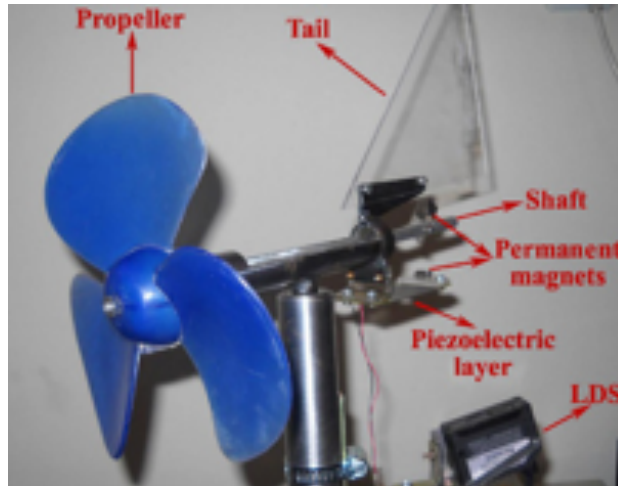
Fig. 35.1: The piezoelectric wind energy harvester (PWEH).
