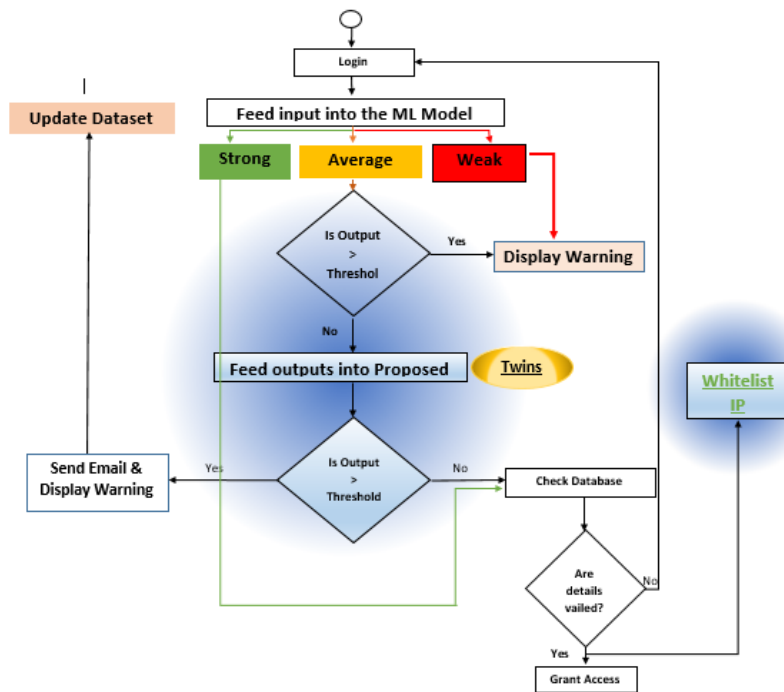
Fig. 8 Workflow of the proposed method in application layer
