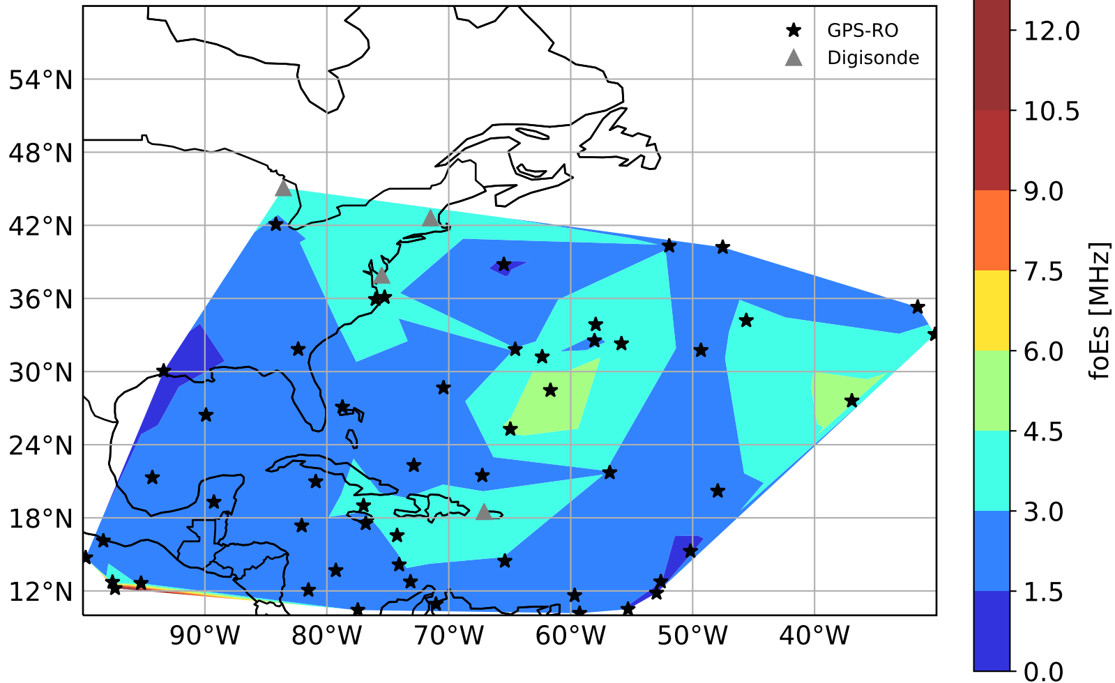
Es Measurements 3:00-6:00 UTC Jul 13
