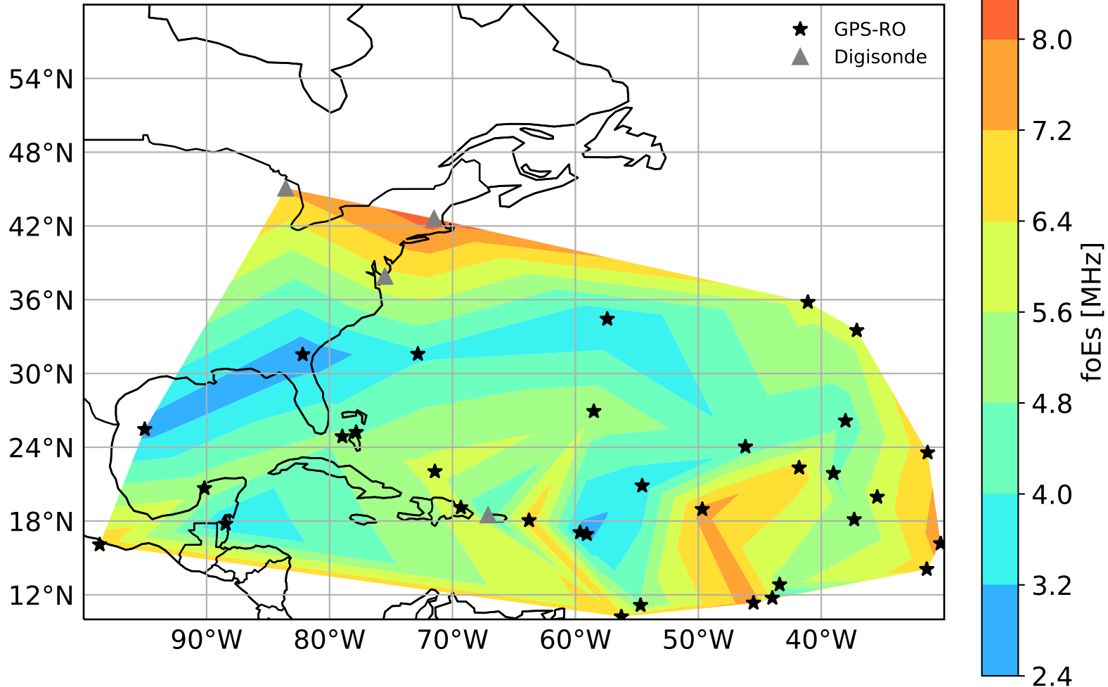
Es Measurements 15:00-18:00 UTC Jul 14
