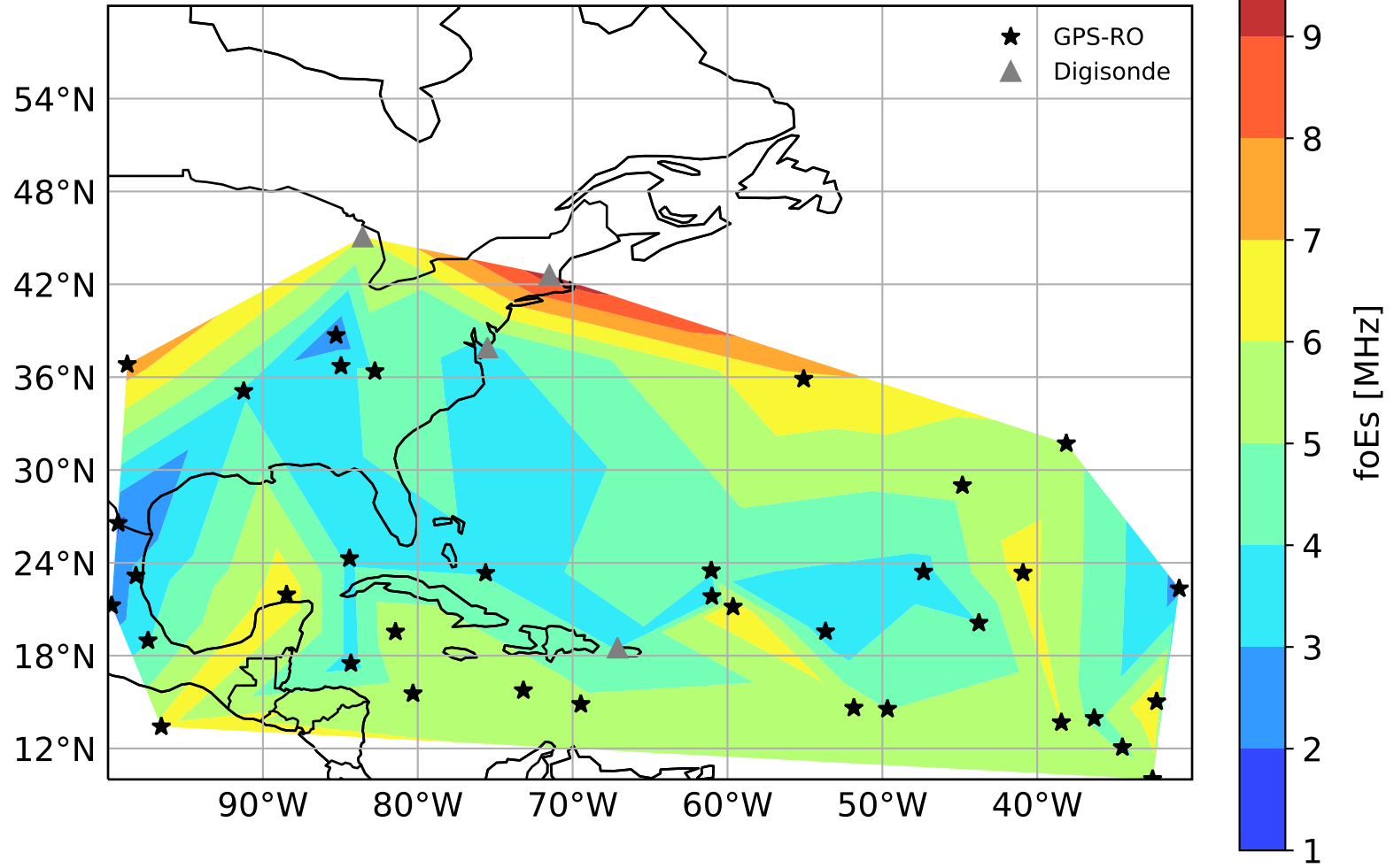
Es Measurements 12:00-15:00 UTC Jul 15
