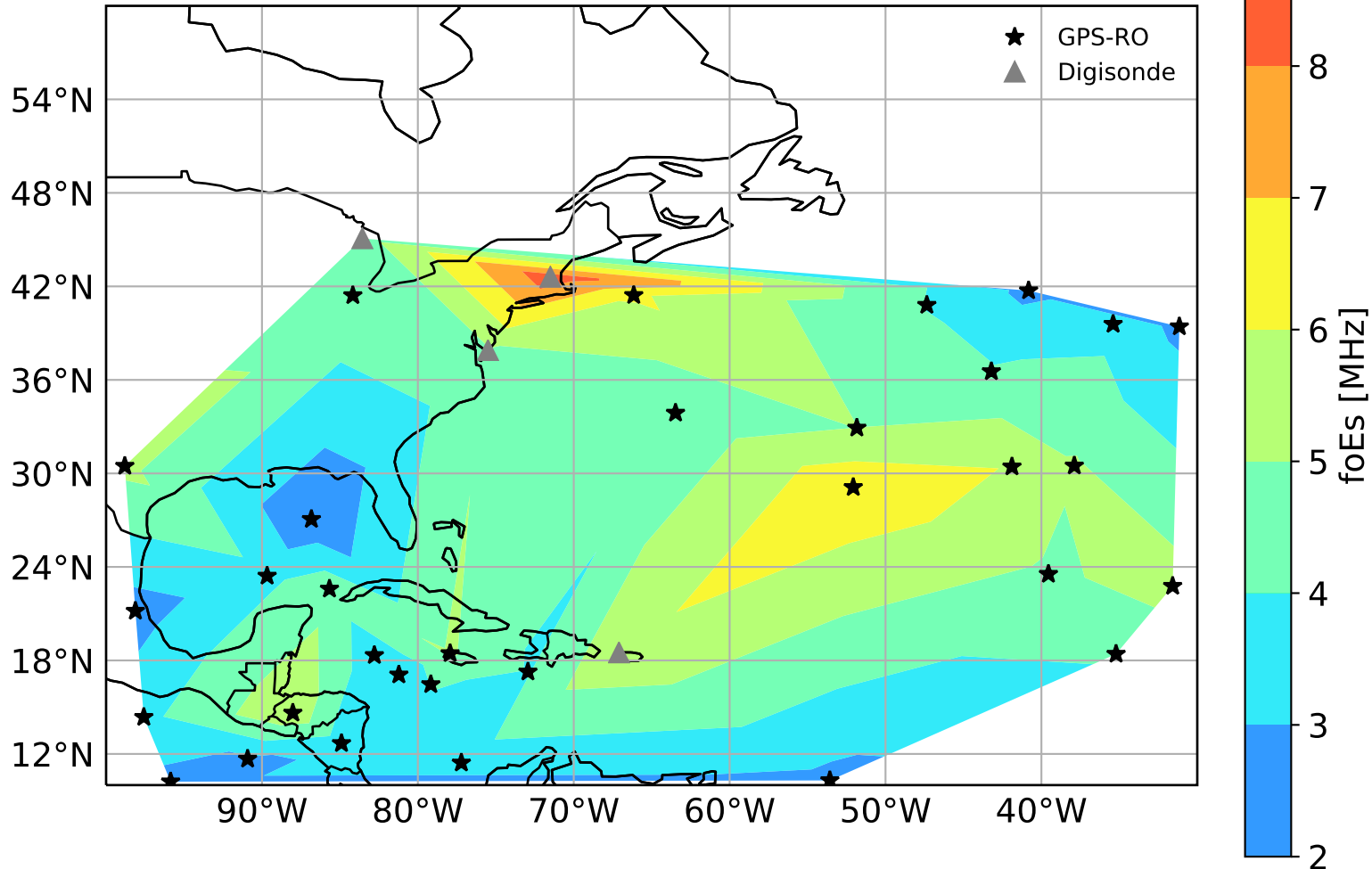
Es Measurements 0:00-3:00 UTC Jul 13
