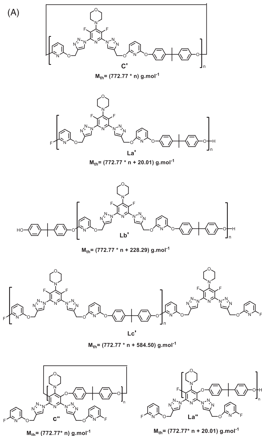
FIGURE 3 (A) Possible reaction products of P1 obtained after polycondensation of monomer (6) with BPA. (B) MALDI-TOF mass spectrum of P1
