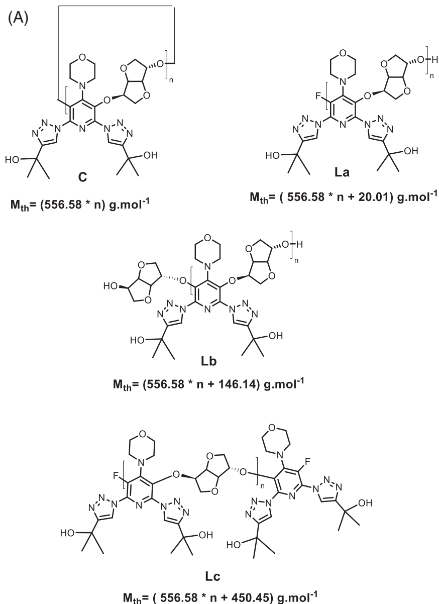
FIGURE 6 (A) Possible reaction products of P4 obtained after polycondensation of monomer (7) with ISB. (B) MALDI-TOF mass spectrum of P4
