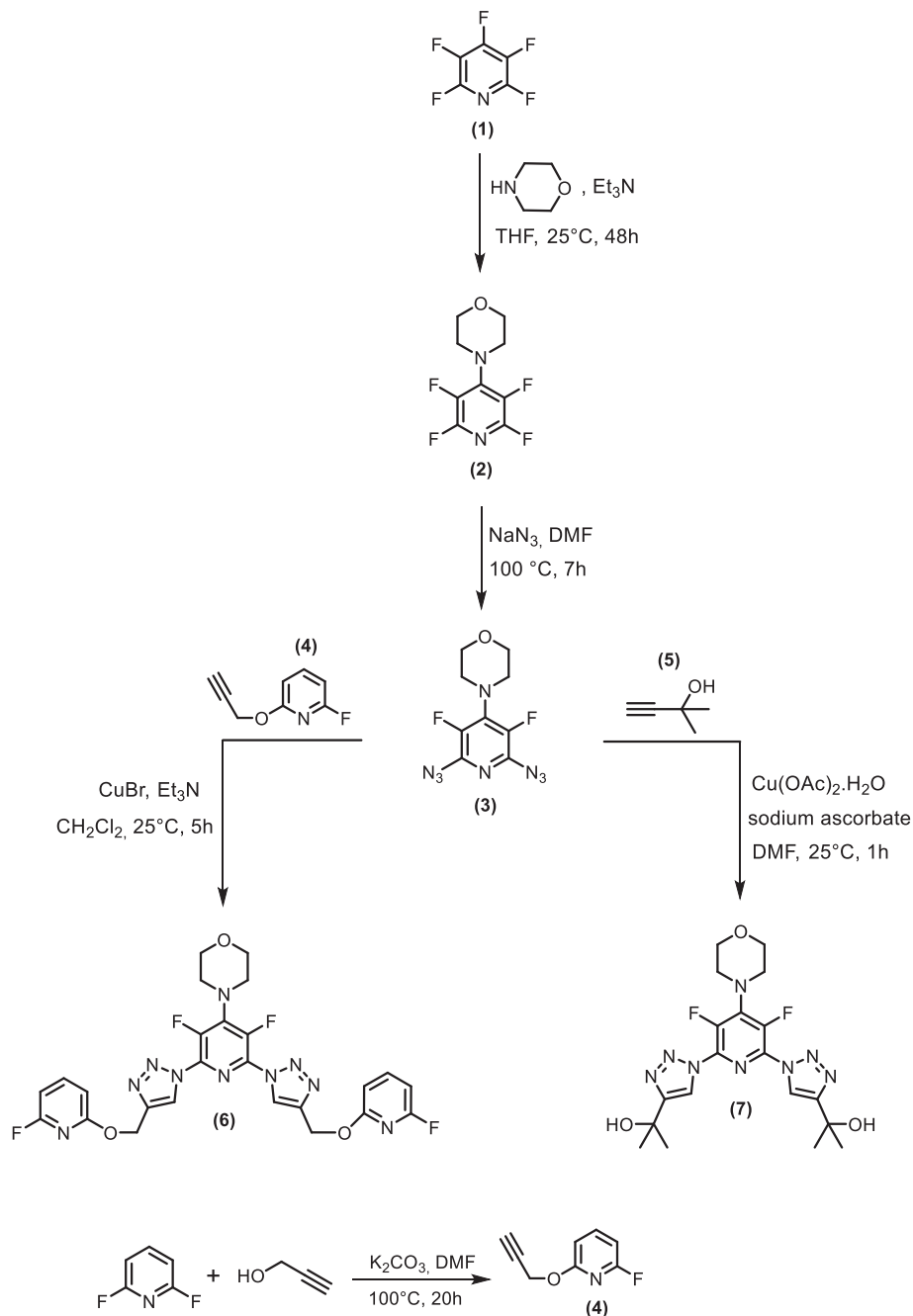
SCHEME 1 Synthesis of 1,2,3-triazole-based fluorinated monomers (6–7).
