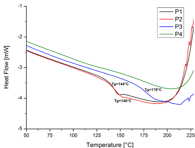
FIGURE 8 Differential scanning calorimetry curves of polymers P1-P4
