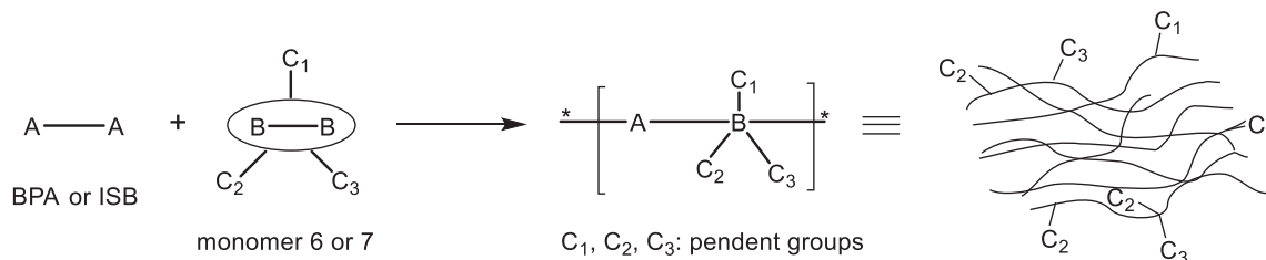
FIGURE 10 Representative scheme of resulting polymers with effects of entanglements and pendent group structures.
