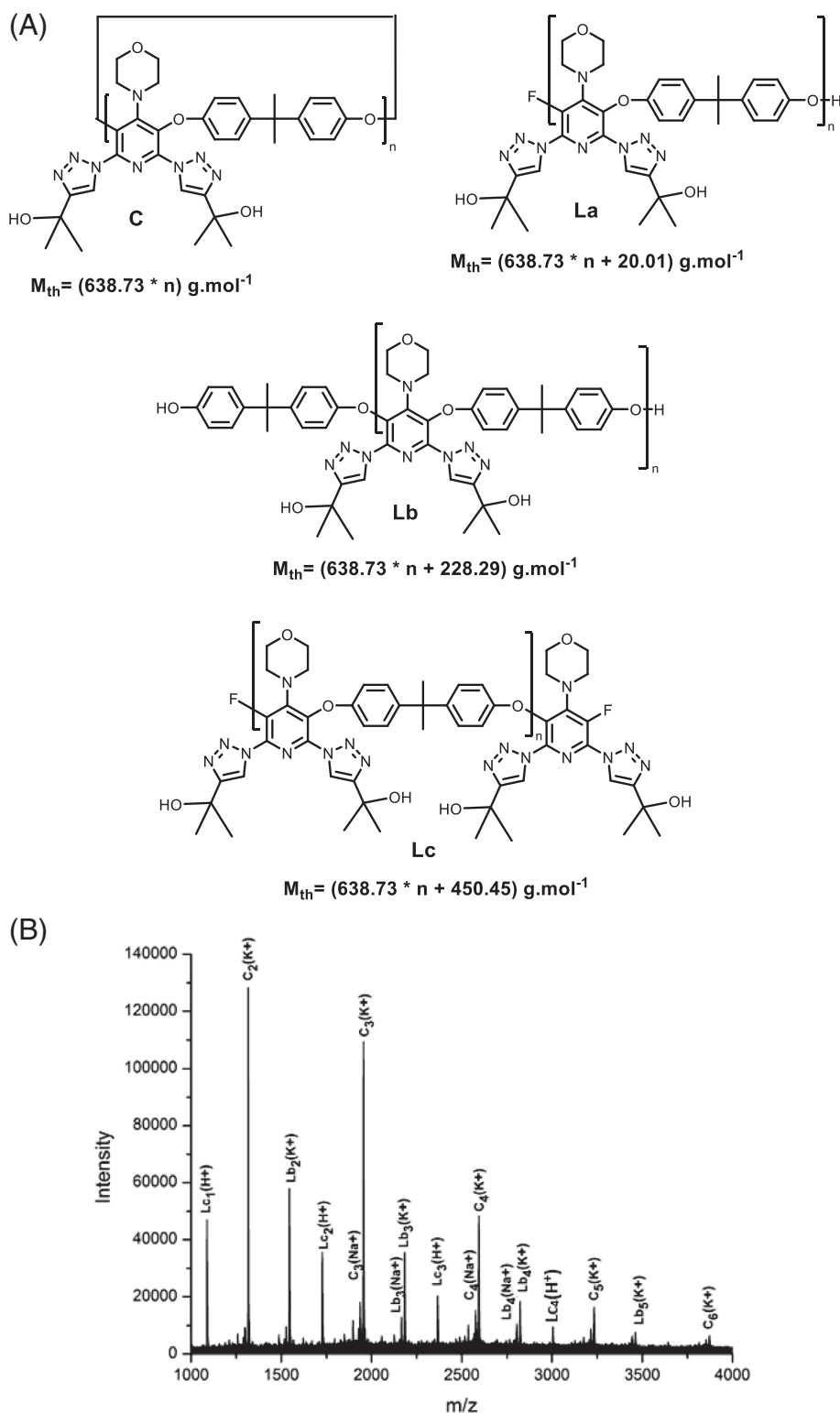
FIGURE 5 (A) Possible reaction products of P3 obtained after polycondensation of monomer (7) with BPA. (B) MALDI-TOF mass spectrum of P3
