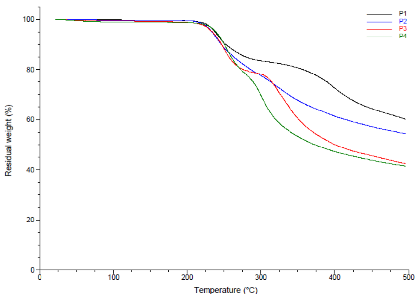
FIGURE 9 Thermogravimetric analysis traces of polymers P1-P4
