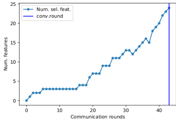
Fig. 6: FFS process on MAV dataset.
