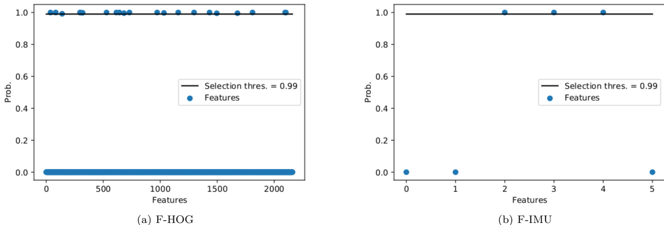
Fig. 5: FFS probability for HOG and IMU. The selected features are those with probability greater than 0.99 (above threshold).
