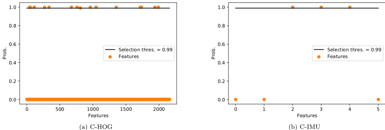
Fig. 4: Centralised FS probability for HOG and IMU. The selected features are those with probability greater than 0.99 (above threshold).
