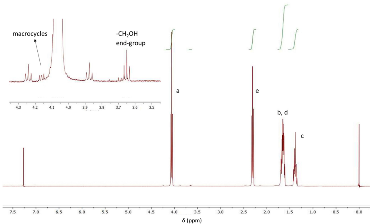
Figure S3b. ^1\text{H} NMR of PCL6500D after incubation with cutinase (1.5 h).
