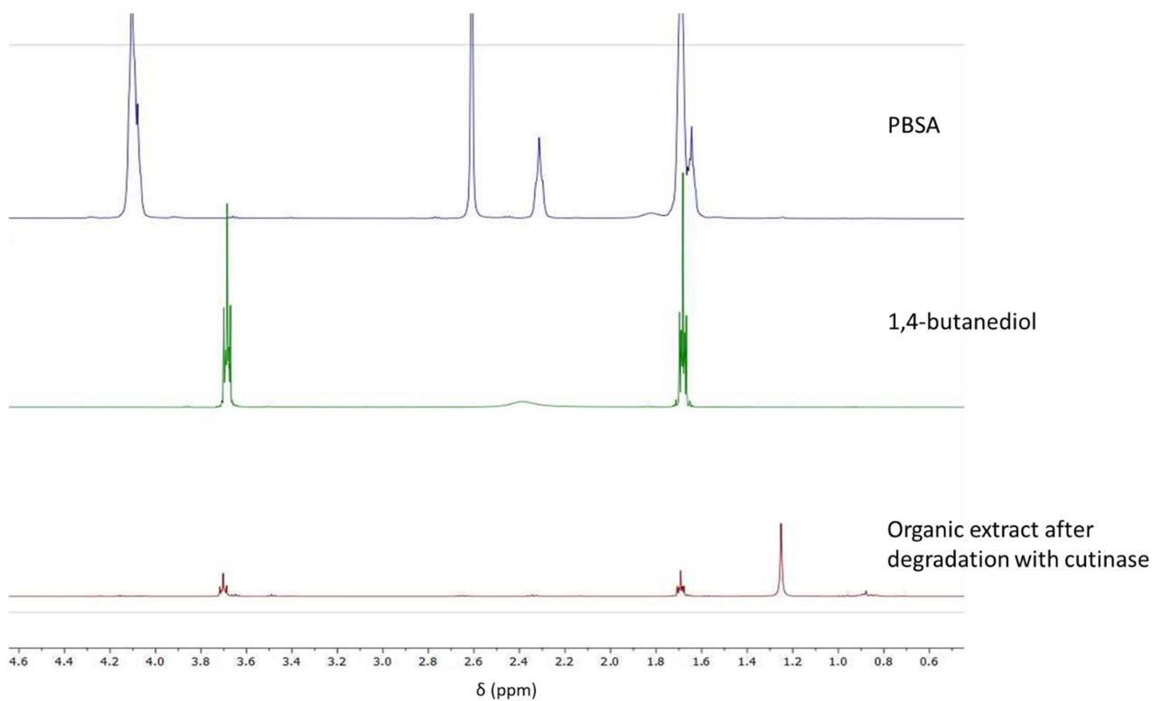
Figure S2c. 1 H NMR of the organic extract after degradation of PBSA with cutinase, compared to pristine PBSA and 1,4-butanediol.
