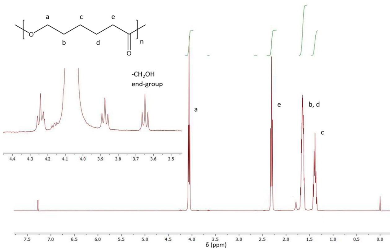
Figure S3a. 1 H NMR of PCL (6500D and 6800D).
