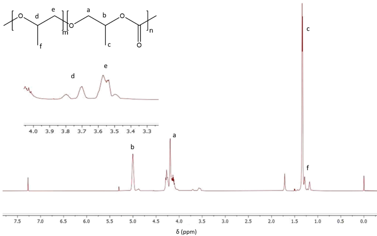
Figure S5a. ^1\text{H} NMR of PPC.
