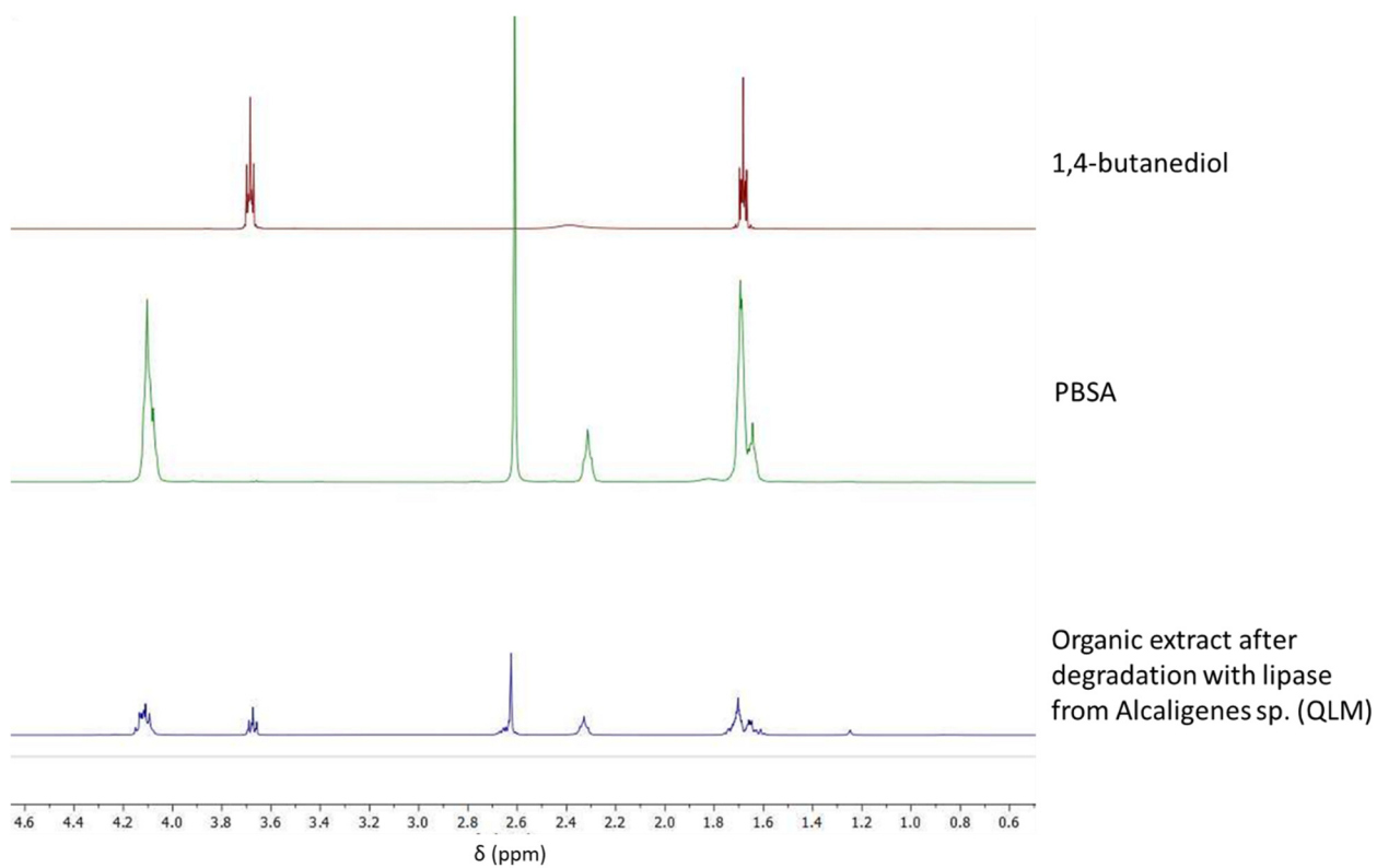
Figure S2e. 1 H NMR of the organic extract after degradation of PBSA with lipase from Alcaligenes sp. (QLM), compared to pristine PBSA and 1,4-butanediol.
