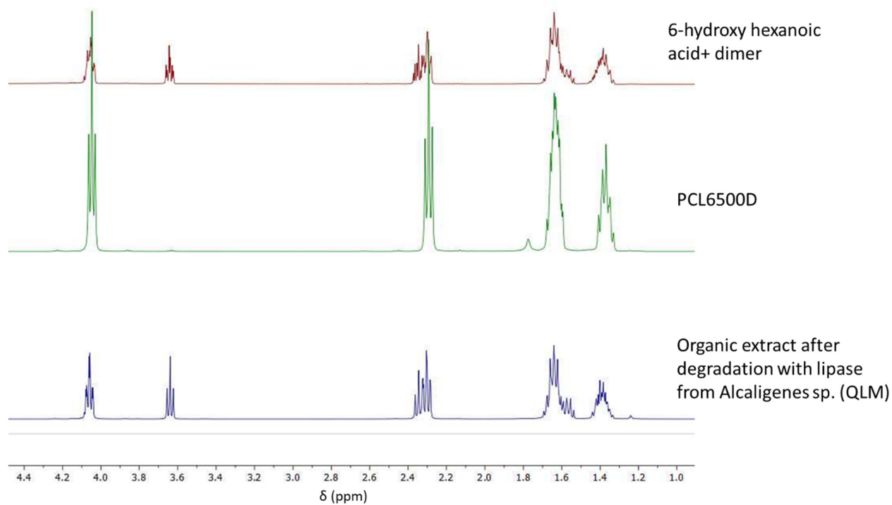
Figure S3f. 1 H NMR of the organic extract after degradation of PCL6500D with lipase from Alcaligenes sp. (QLM), compared to pristine PCL6500D and 6-hydroxyhexanoic acid.
