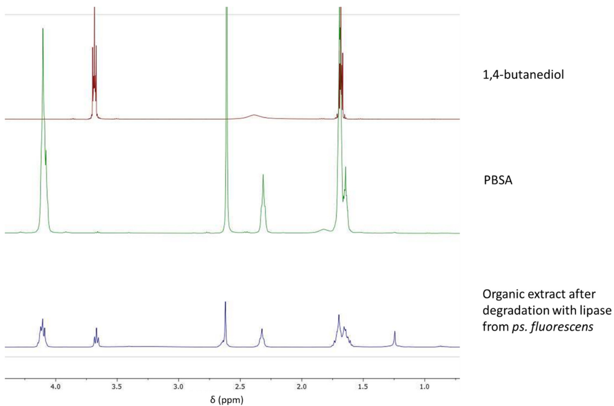
Figure S2d. 1 H NMR of the organic extract after degradation of PBSA with lipase from ps. fluorescens , compared to pristine PBSA and 1,4-butanediol.
