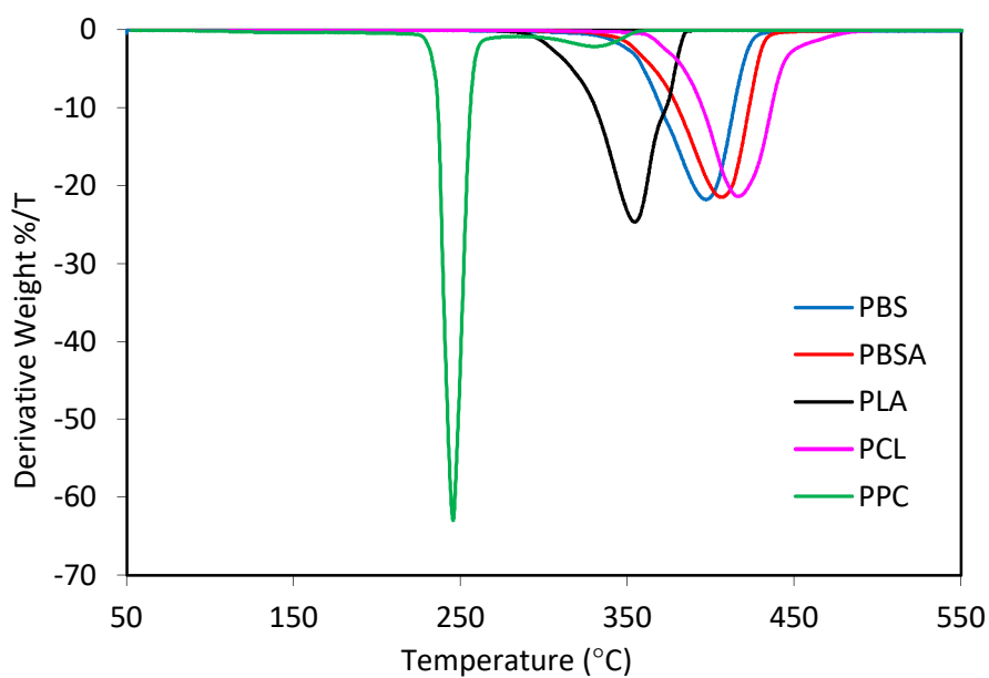
Figure S7b. dTGA curves of polyesters.
