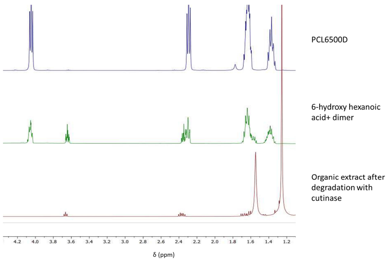
Figure S3c. ^1\text{H} NMR of the organic extract after degradation of PCL6500D with cutinase, compared to pristine PCL6500D and 6-hydroxyhexanoic acid.
