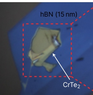
(a) Optical image
