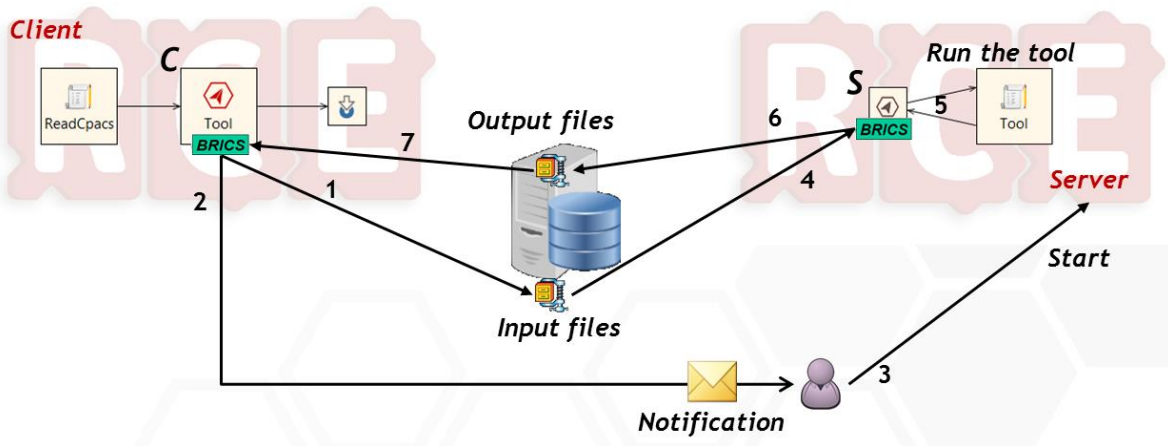
Fig. 5 Schematic representation of the Brics protocol in the context of a client and a server workflow in RCE. The numbered arrows indicate the steps taken to accomplish the remote execution, as described in the text above.
