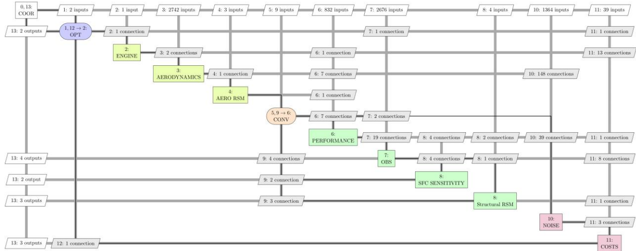
Fig. 12 AGILE 4.0 AC6 MDAO XDSM of the MDAO workflow.
