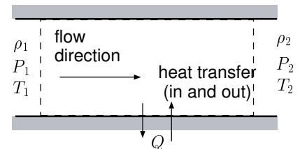
Fig. 14.39 – The control volume of Rayleigh Flow.
