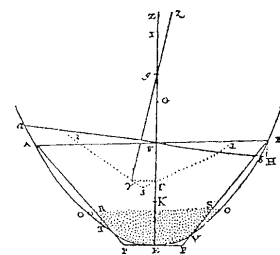
Fig. 4.41 – Bouguer Showing Meta-center.
