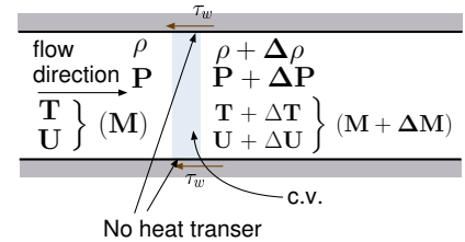
Fig. 14.19 – Control volume of the gas flow in a pipe. The flow is assumed to be relatively short.
