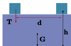
Fig. 4.59 – Measurement of GM — of floating body. M_{weight} = T d (4.165)
