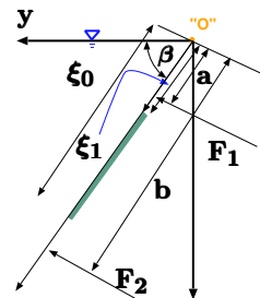
Fig. 4.22 – The general forces acting on submerged area.
