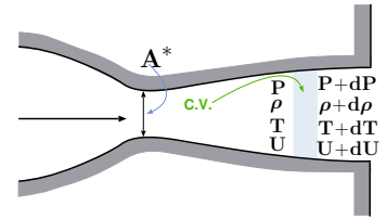
Fig. 14.7 – Control volume inside a converging-diverging nozzle.
