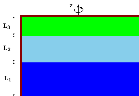
Fig. 4.65 – Three liquids layers under rotation with various critical situations.
