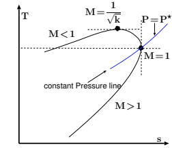
Fig. 14.40 – The temperature entropy diagram for Rayleigh line.
