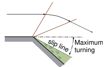
Fig. 15.25 - Expansion of Prandtl-Meyer function when it exceeds the maximum angle.
