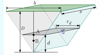
Fig. 4.51 – Floating upside down triangle in liquid. The Points A and B are representation to actual location which is at the center.
