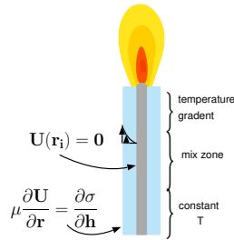
Fig. 8.15 – Flow in a kandle with a surface tension gradient.
