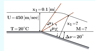
Fig. 15.29 – Schematic for Example 15.16.
