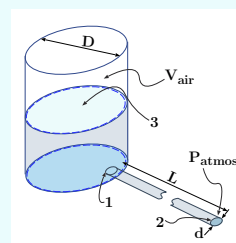
Fig. 7.7 – Liquid exiting a large tank through a long tube.
