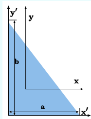
Fig. 3.17 – Product of inertia for triangle.
