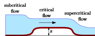
Fig. 17.13 – Transition from subcritical to supercritical. The curves are not to scale.
