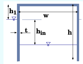
Fig. 4.37 – Schematic of a thin wall floating body.
