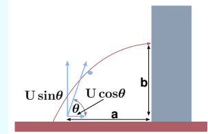
Fig. 3.1 – Description of the extinguish nozzle aimed at the building window.
