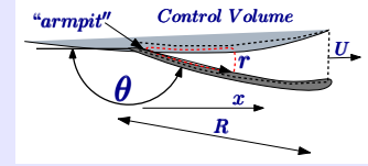
Fig. 5.6 – Pectoral fin control volume for the analysis of the velocity. The red dashed line reprered the smass control volume.
