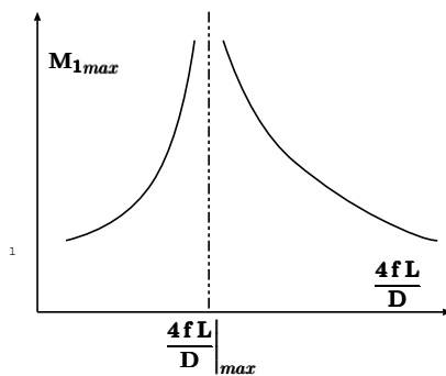
(b) The maximum entrance Mach number, M_1 to the tube as a function of \frac{4fL}{D} supersonic branch.
