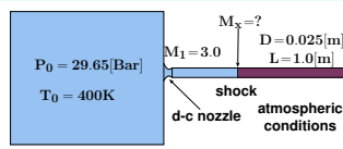
Fig. 14.22 – The schematic of Example (14.19).
