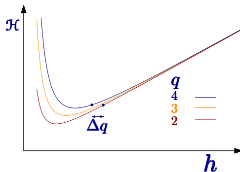
Fig. 17.21 – Flow in contraction subcritical flow. The specific energy in diagram is \mathcal{H} = 3 . The flow at section 1 with q_1 increase the flow rate per width to section 2. At section 2 now the flow rate is given and with specific energy \mathcal{H} all the parameters can be found. For example in
