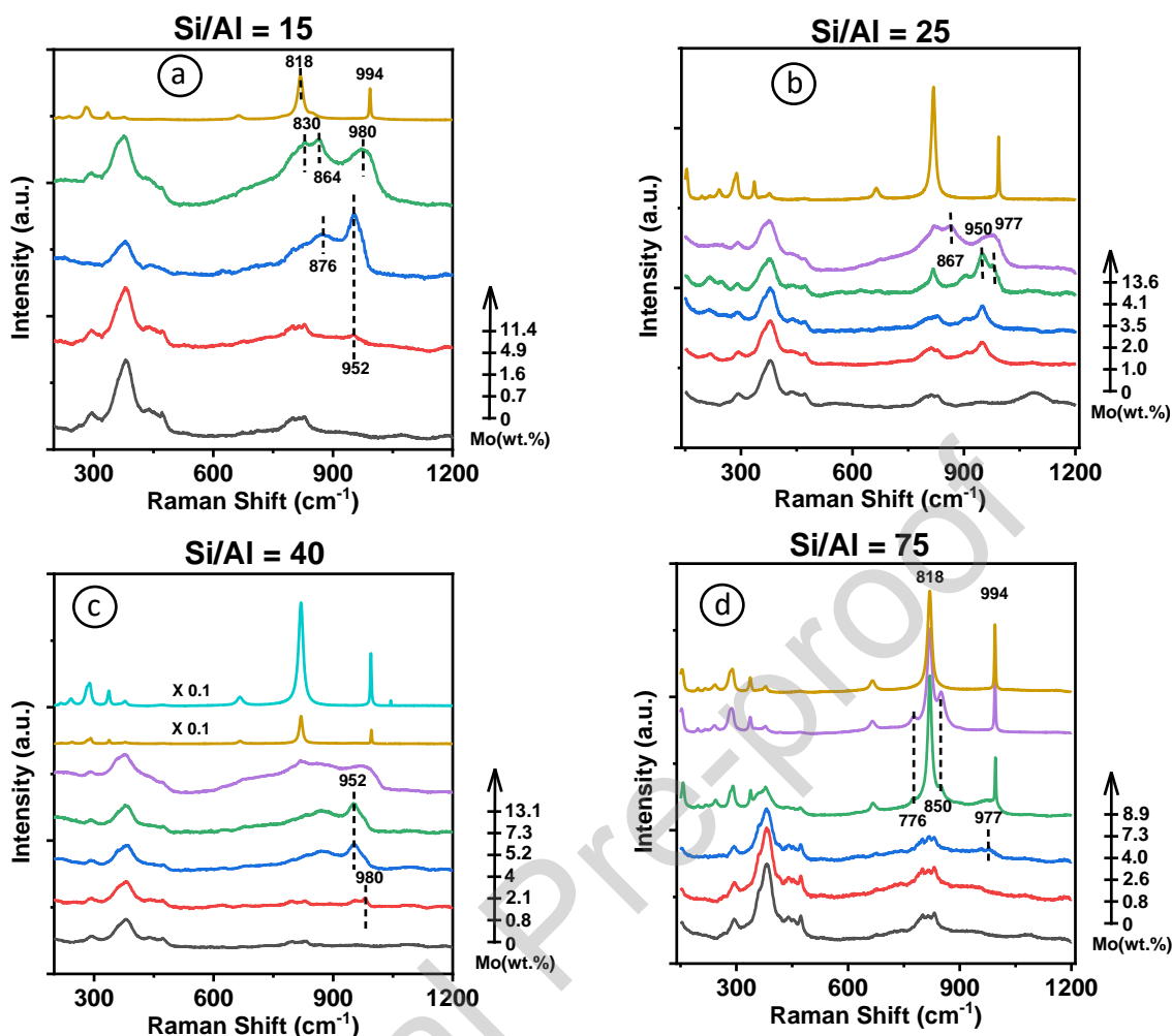
Figure 3: Raman spectra of the calcined catalysts as a function of the Mo loading for the different catalyst series: (a) Si/Al = 15; (b) Si/Al = 25; (c) Si/Al = 40 and (d) Si/Al = 75.
