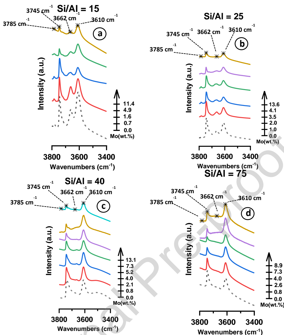
Figure 4: IR spectra of OH region of the calcined catalysts as a function of the Mo loading for the different catalyst series: (a) Si/Al = 15; (b) Si/Al = 25; (c) Si/Al = 40 and (d) Si/Al = 75. The spectra intensity was normalized from the zeolite amount.
