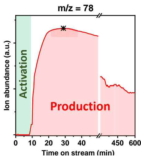
Figure 6: Mass spectra of the benzene as a function of time on stream. The red area corresponds to the cumulative yield of benzene and is possible to separate into two parts. Before (*) refers to the induction period and after (*) to the deactivation step.
