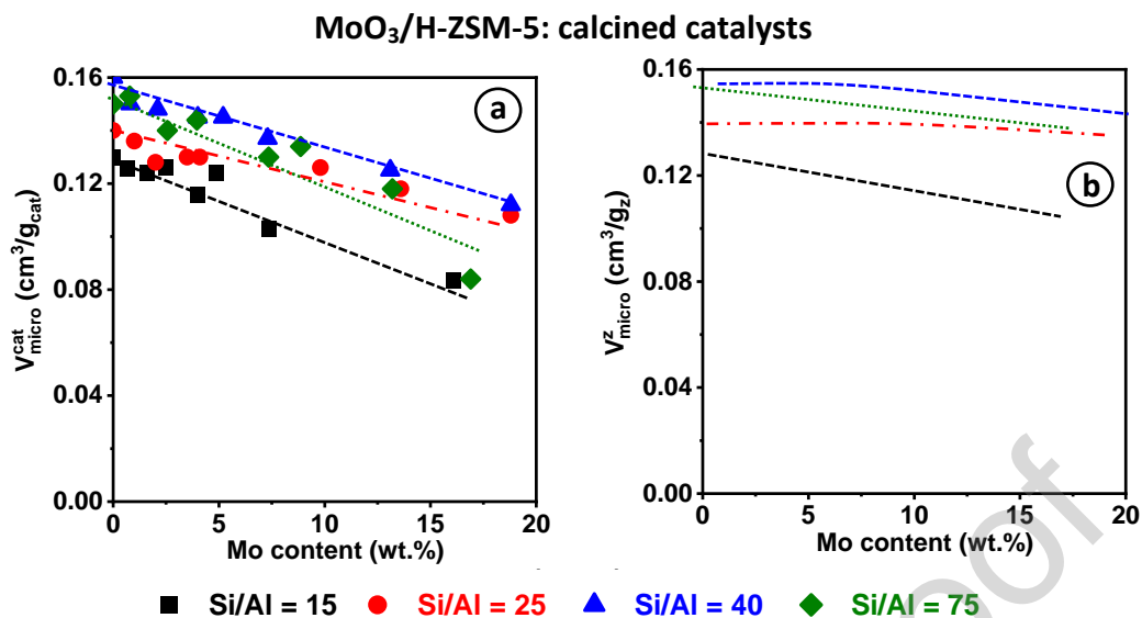
Figure 2: Microporous volume per catalyst weight V_{micro}^{cat} (a) and per zeolite weight V_{micro}^z (b) as a function of the Mo loading for the different catalyst series.
