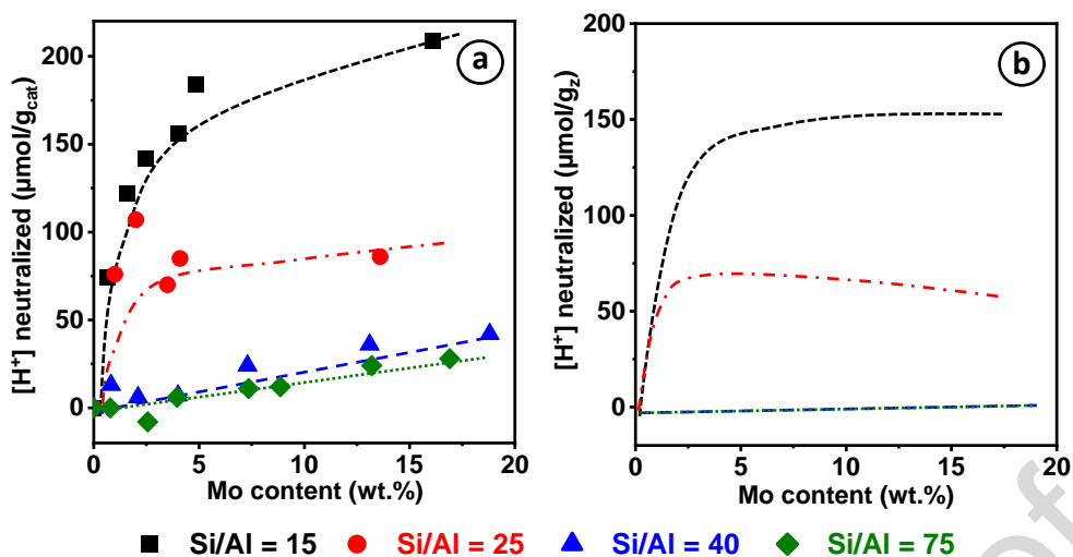
Figure 5: Amount of Brønsted acid sites neutralized after Mo impregnation as a function of the Mo loading for the different series of catalysts. The data in full and open symbols are normalized from the amount of catalyst (a) and zeolite (b), respectively.
