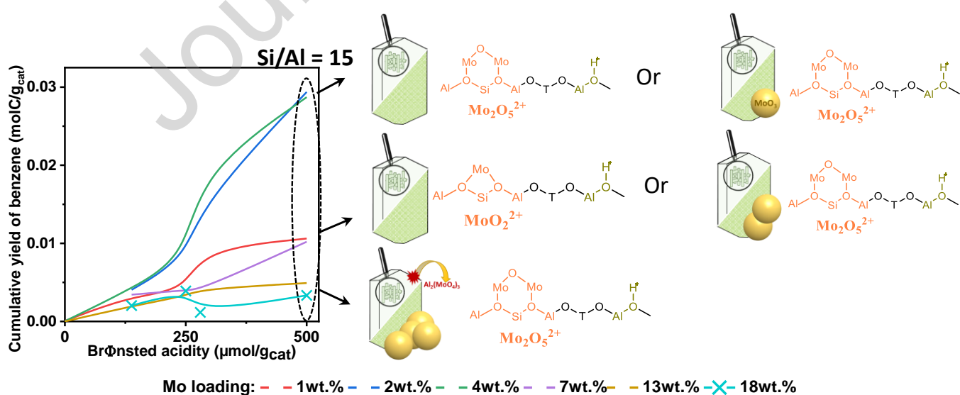
Scheme 2: Cumulative yield of benzene as a function of the initial Brønsted acidity for different Mo loading and establish of a structure-activity relationship for the series Si/Al = 15.
